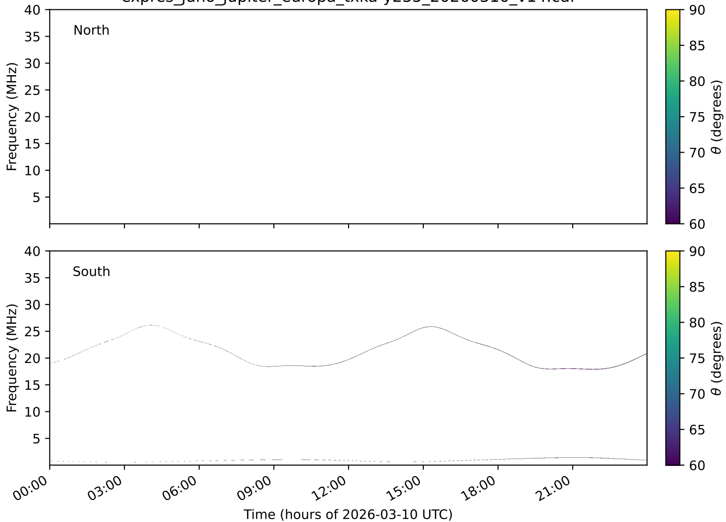
expres_juno_jupiter_europa_txka-y235_20260310_v14.cdf
