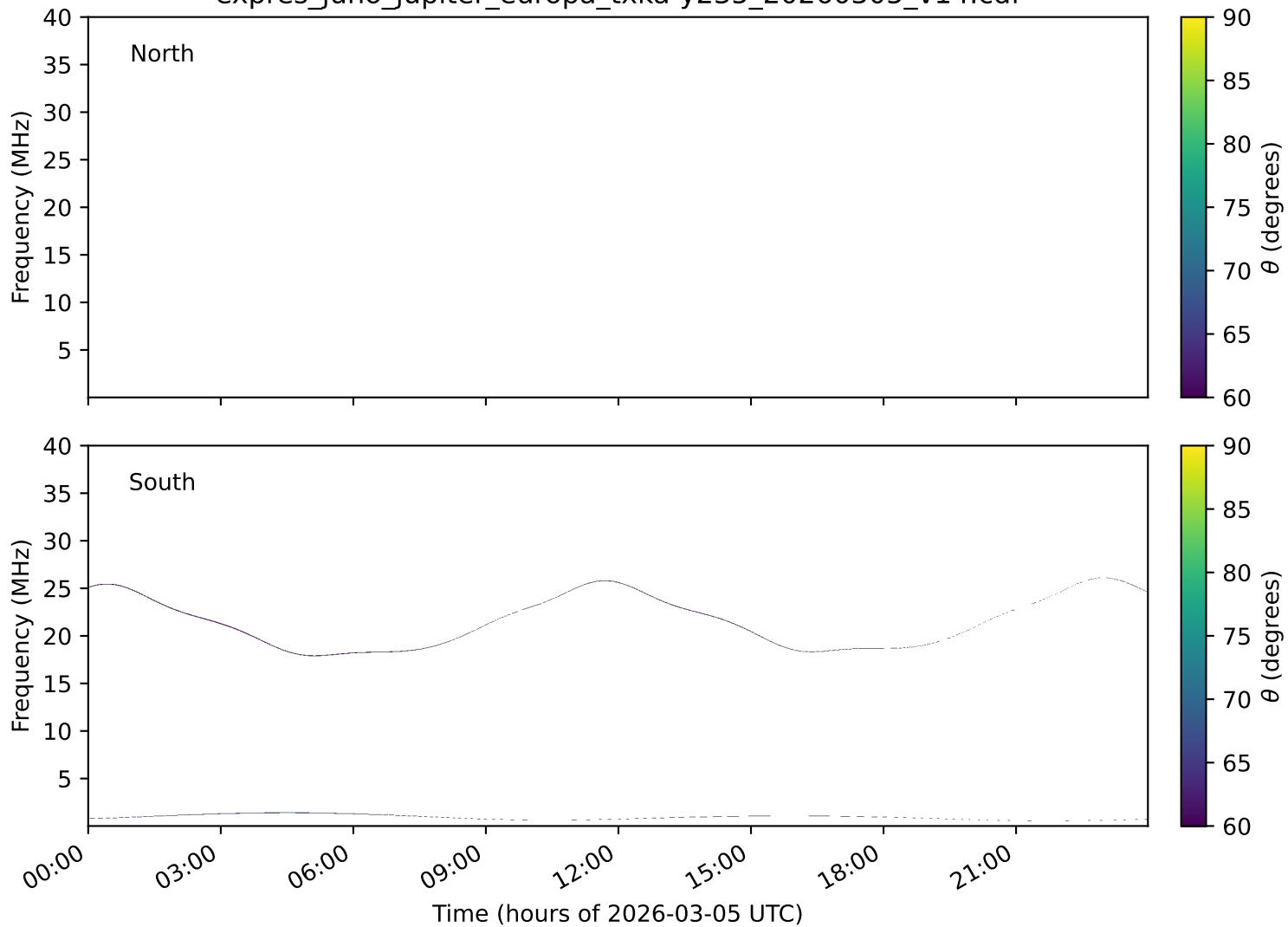
expres_juno_jupiter_europa_txka-y235_20260305_v14.cdf
