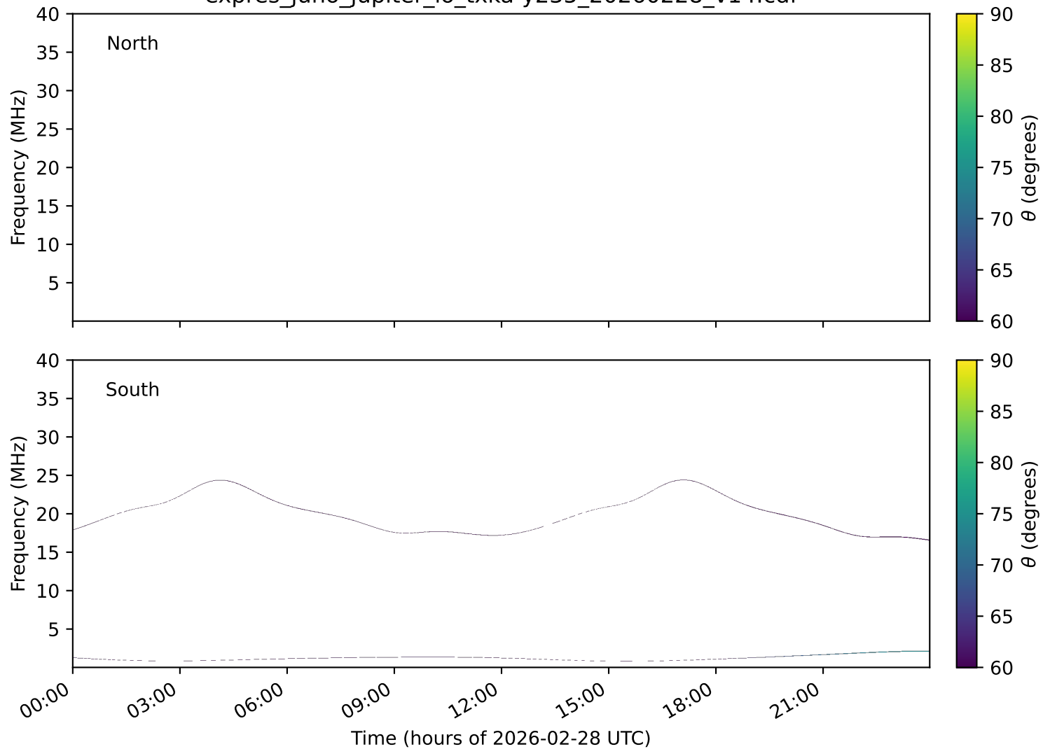
expres_juno_jupiter_io_txka-y235_20260228_v14.cdf
