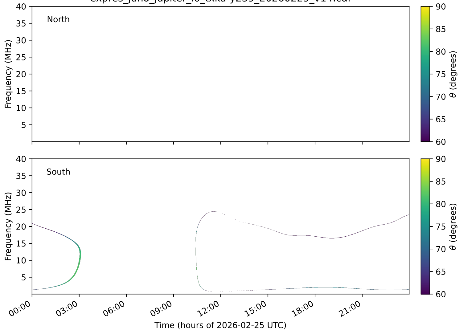
expres_juno_jupiter_io_txka-y235_20260225_v14.cdf
