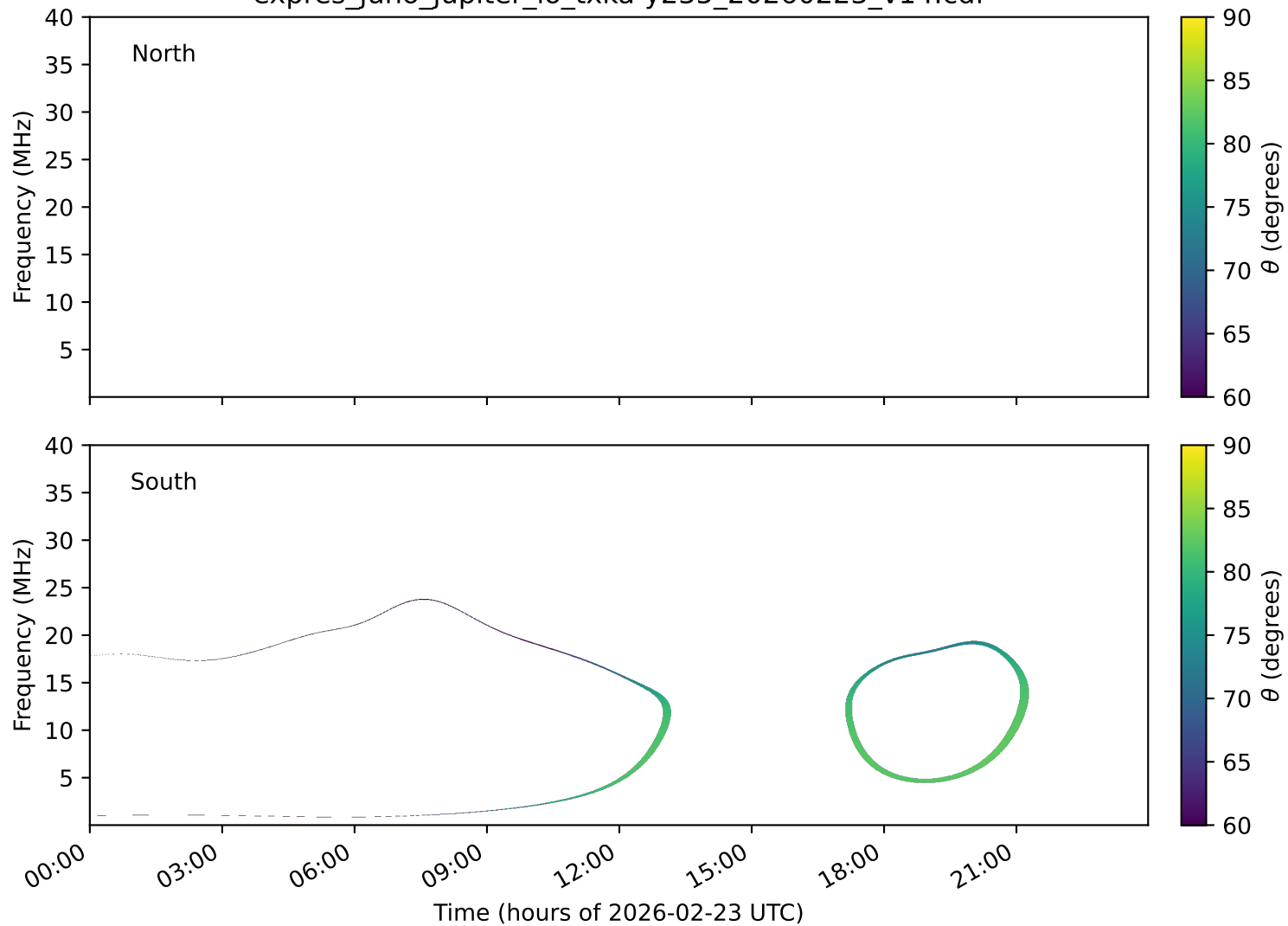
expres_juno_jupiter_io_txka-y235_20260223_v14.cdf
