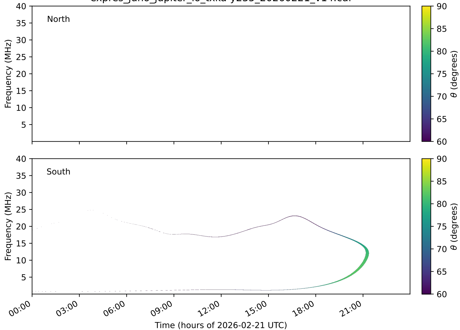
expres_juno_jupiter_io_txka-y235_20260221_v14.cdf
