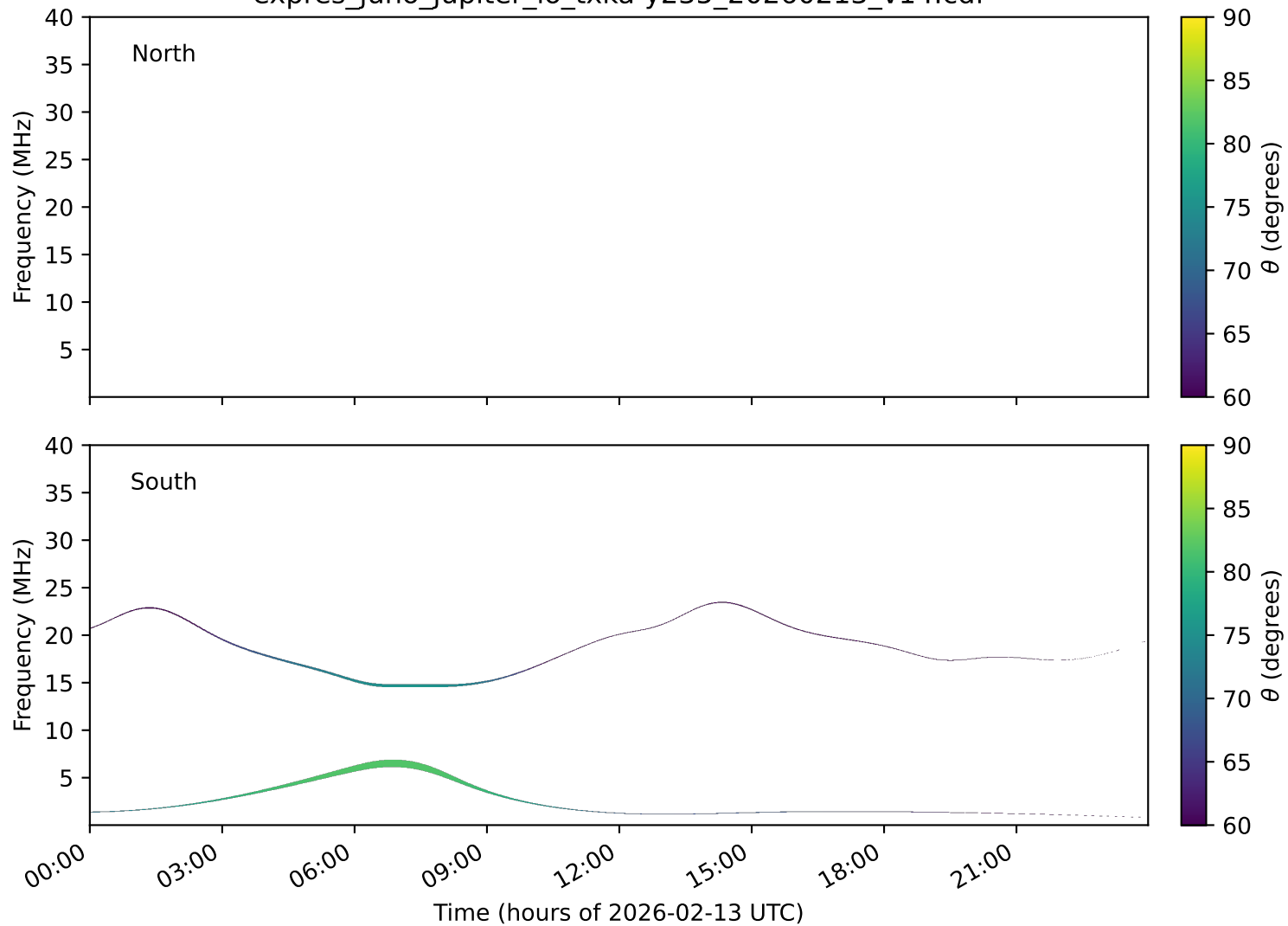
expres_juno_jupiter_io_txka-y235_20260213_v14.cdf
