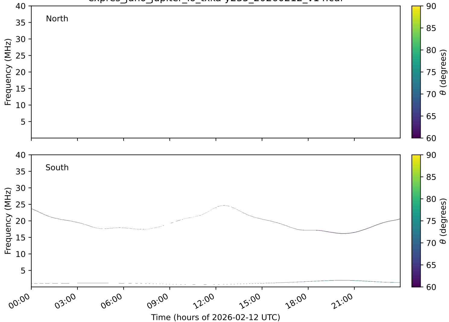
expres_juno_jupiter_io_txka-y235_20260212_v14.cdf
