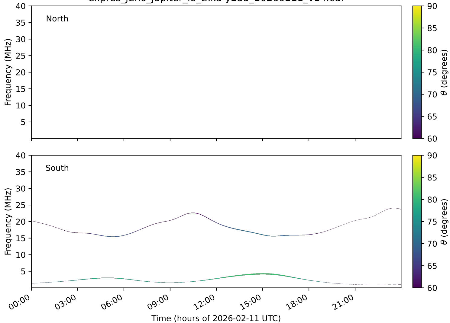
expres_juno_jupiter_io_txka-y235_20260211_v14.cdf
