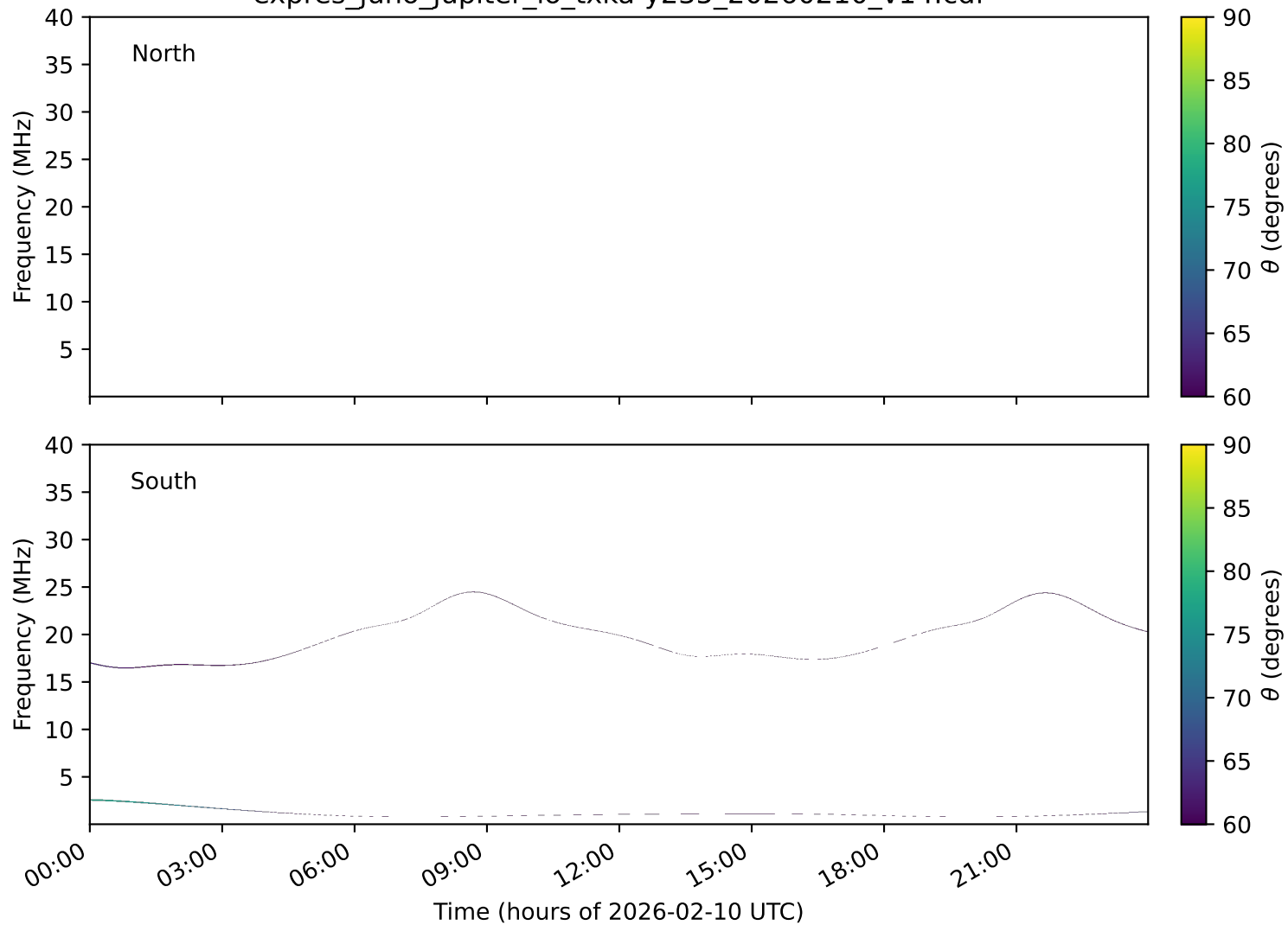
expres_juno_jupiter_io_txka-y235_20260210_v14.cdf
