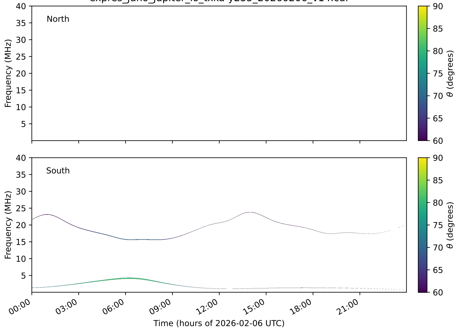
expres_juno_jupiter_io_txka-y235_20260206_v14.cdf
