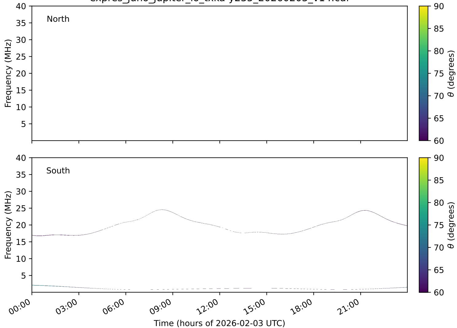
expres_juno_jupiter_io_txka-y235_20260203_v14.cdf
