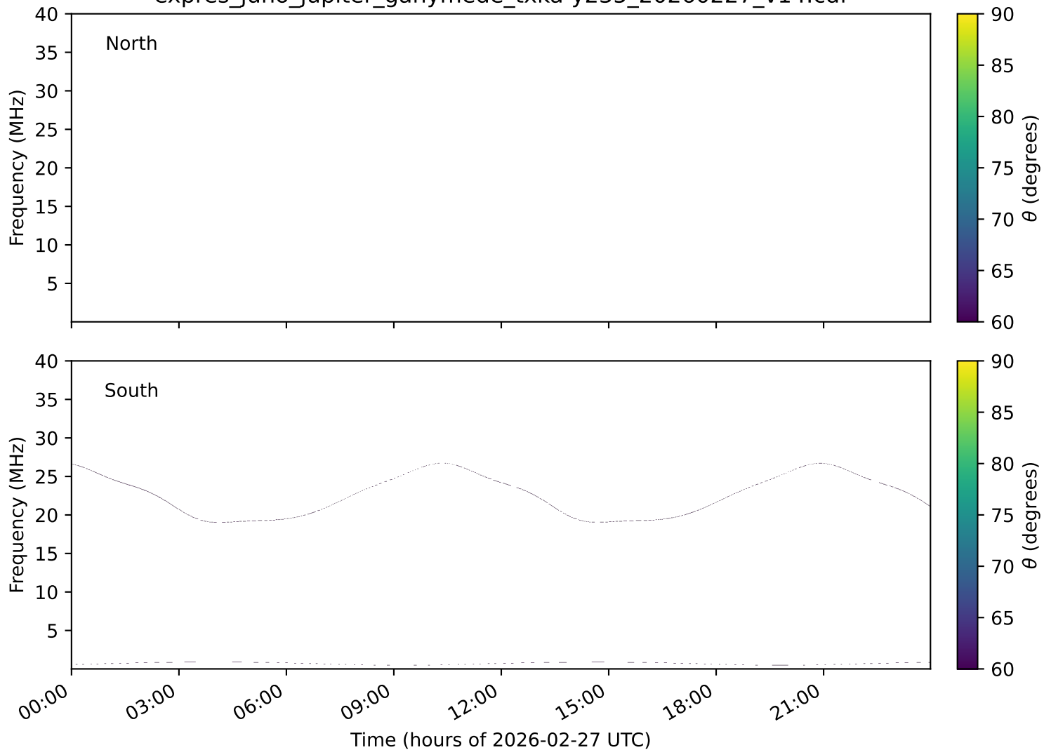
expres_juno_jupiter_ganymede_txka-y235_20260227_v14.cdf
