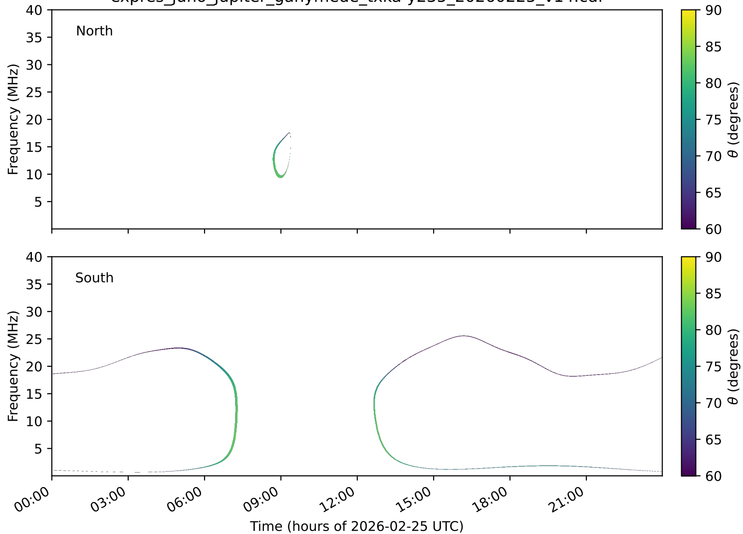
expres_juno_jupiter_ganymede_txka-y235_20260225_v14.cdf
