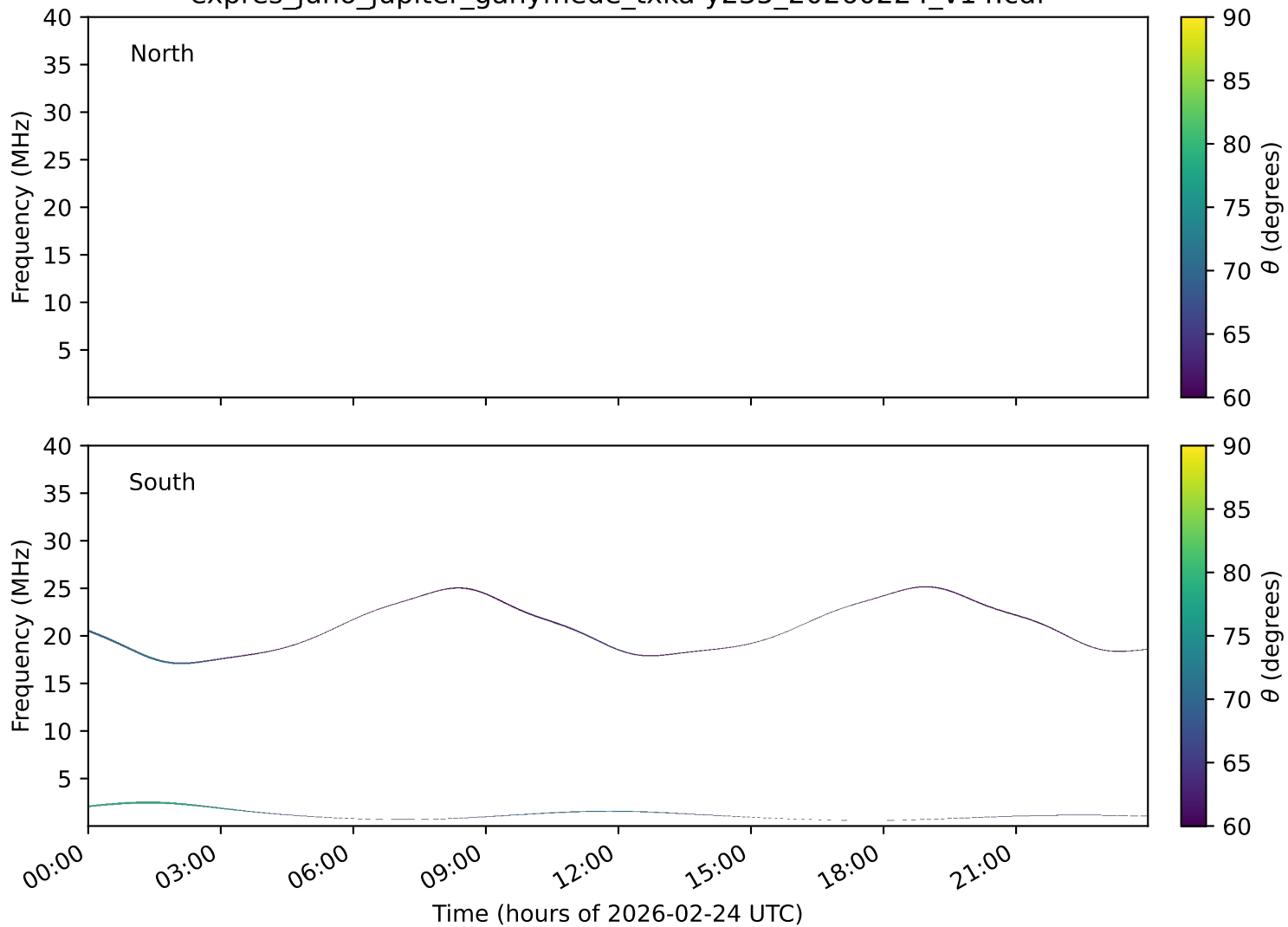
expres_juno_jupiter_ganymede_txka-y235_20260224_v14.cdf
