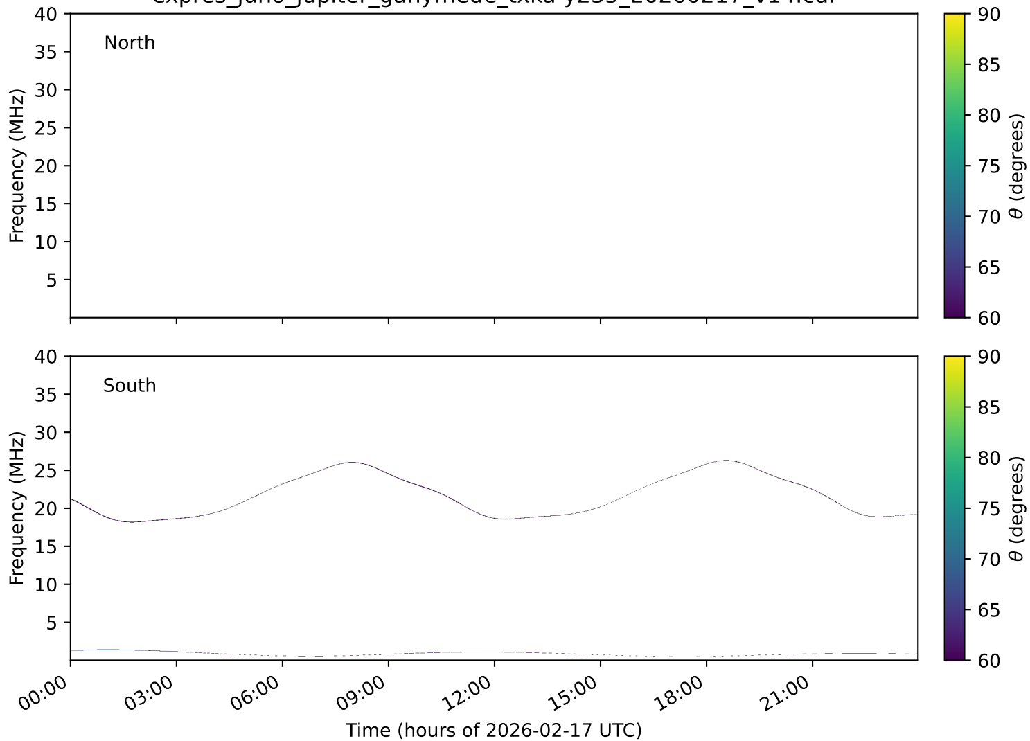
expres_juno_jupiter_ganymede_txka-y235_20260217_v14.cdf
