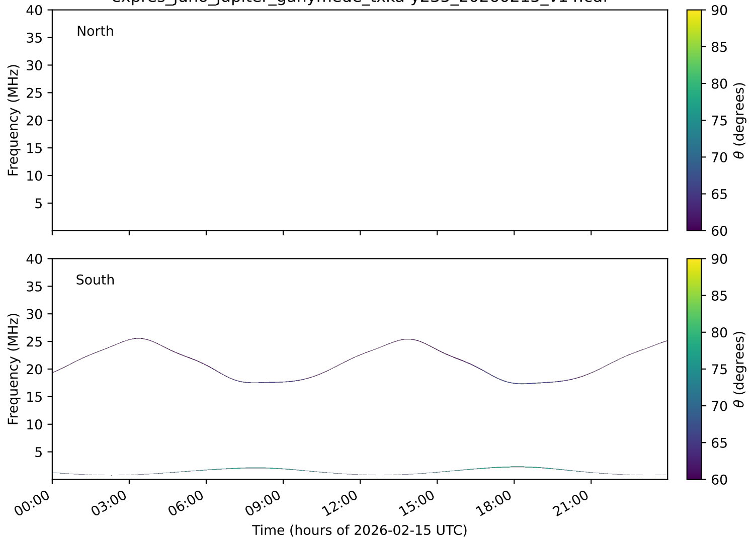
expres_juno_jupiter_ganymede_txka-y235_20260215_v14.cdf
