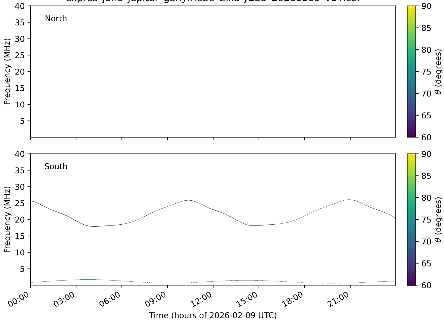
expres_juno_jupiter_ganymede_txka-y235_20260209_v14.cdf
