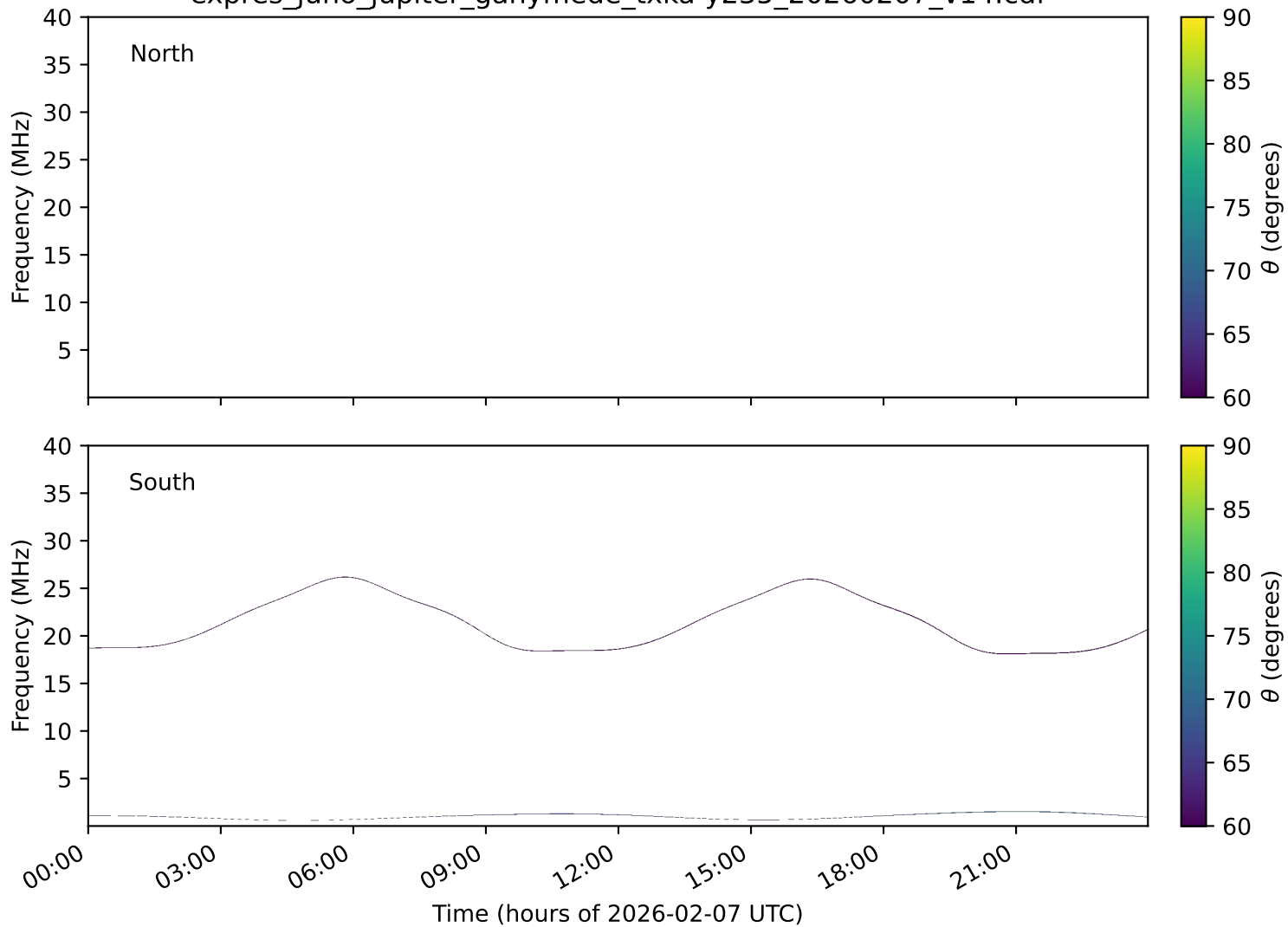
expres_juno_jupiter_ganymede_txka-y235_20260207_v14.cdf
