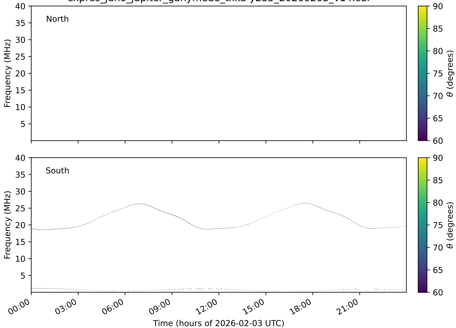
expres_juno_jupiter_ganymede_txka-y235_20260203_v14.cdf
