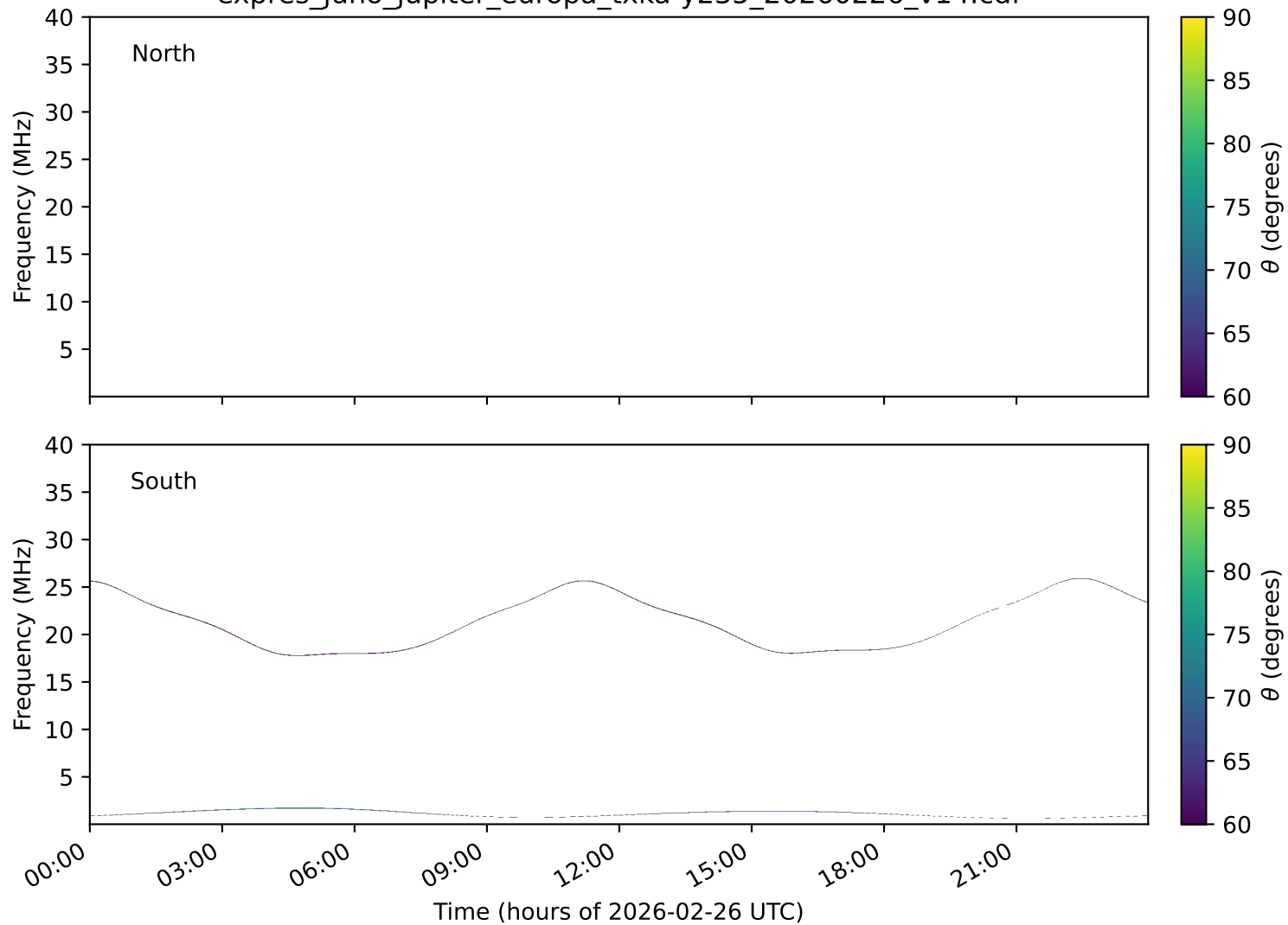
expres_juno_jupiter_europa_txka-y235_20260226_v14.cdf
