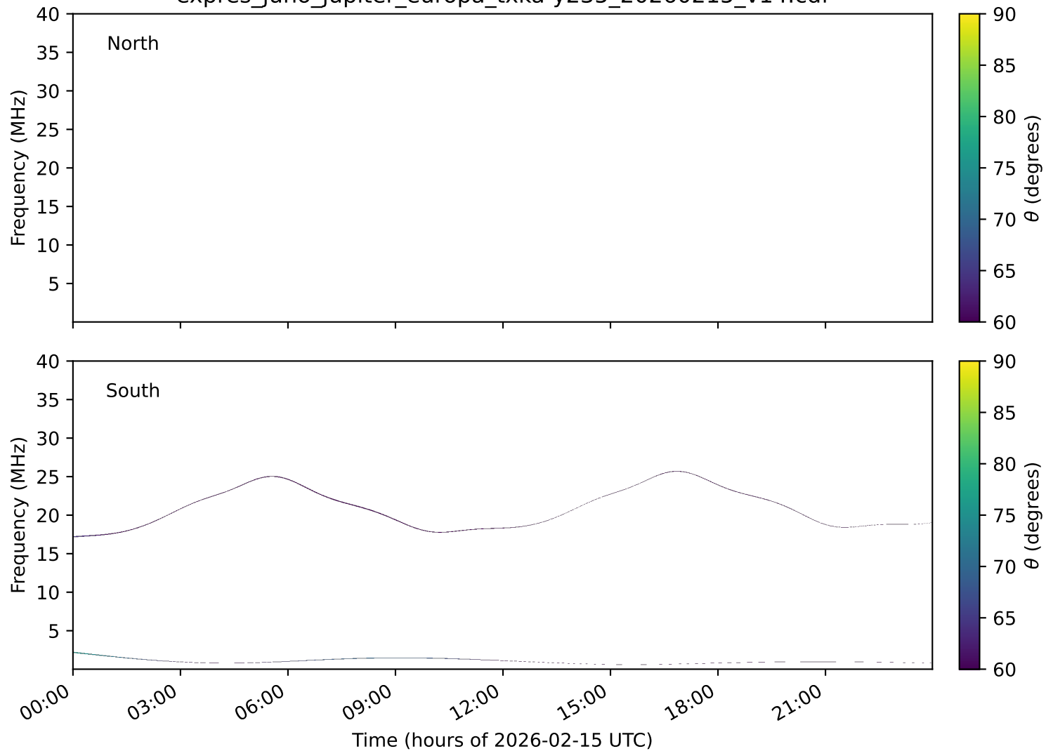
expres_juno_jupiter_europa_txka-y235_20260215_v14.cdf
