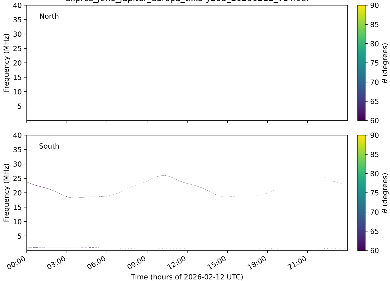
expres_juno_jupiter_europa_txka-y235_20260212_v14.cdf
