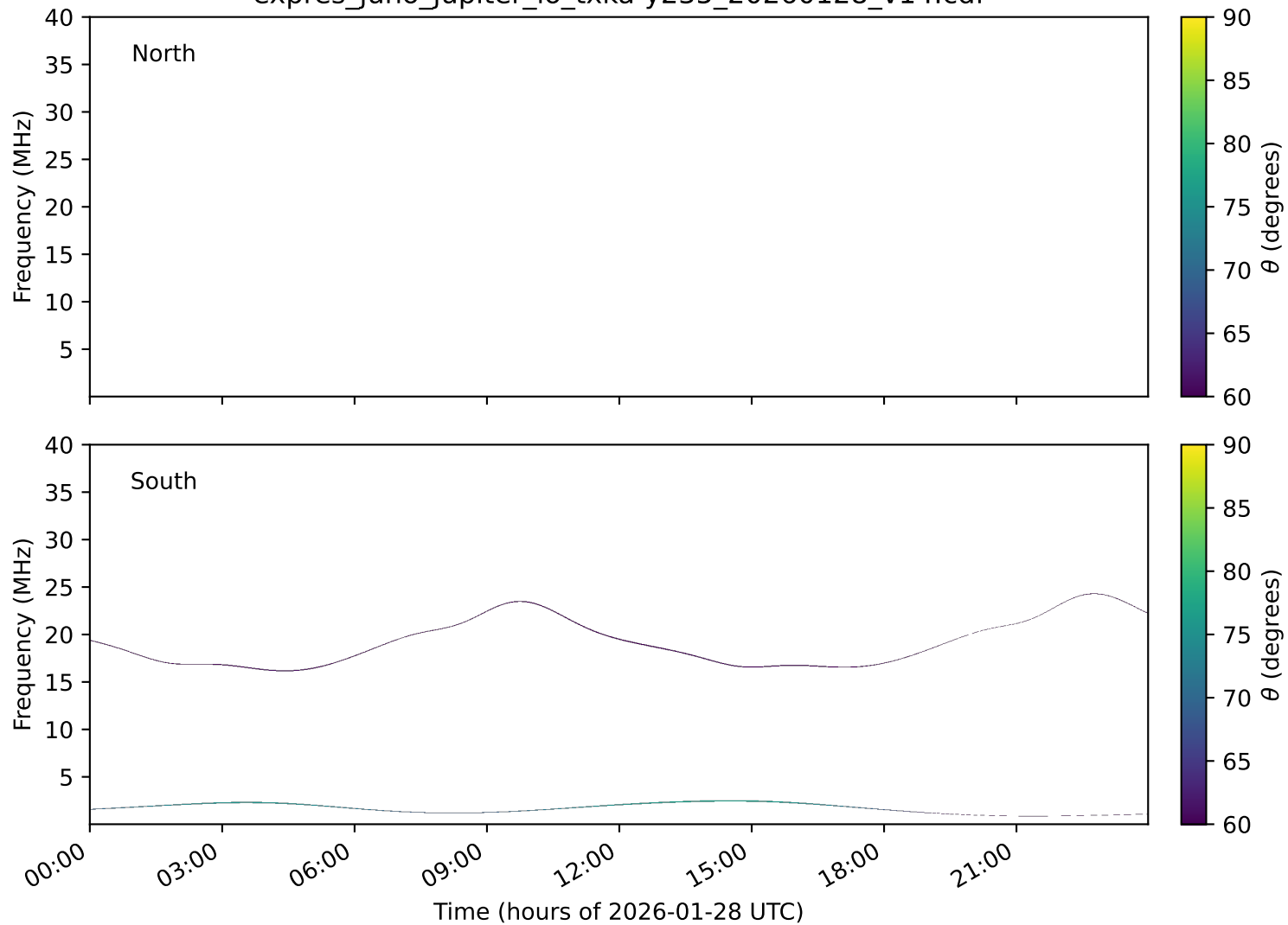
expres_juno_jupiter_io_txka-y235_20260128_v14.cdf
