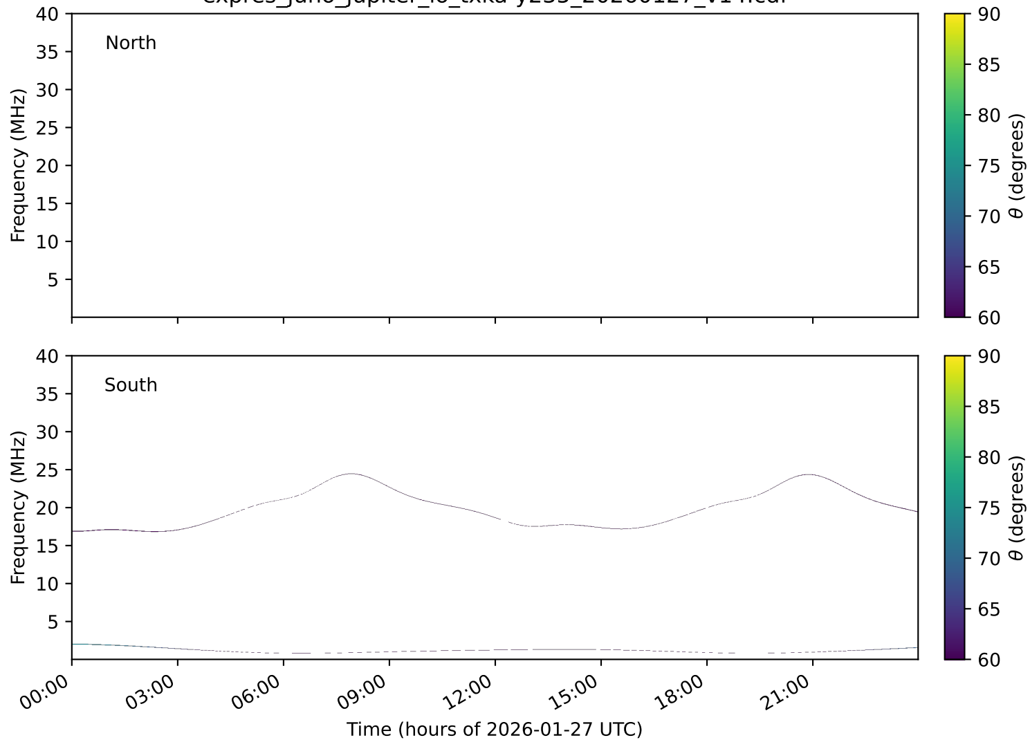
expres_juno_jupiter_io_txka-y235_20260127_v14.cdf
