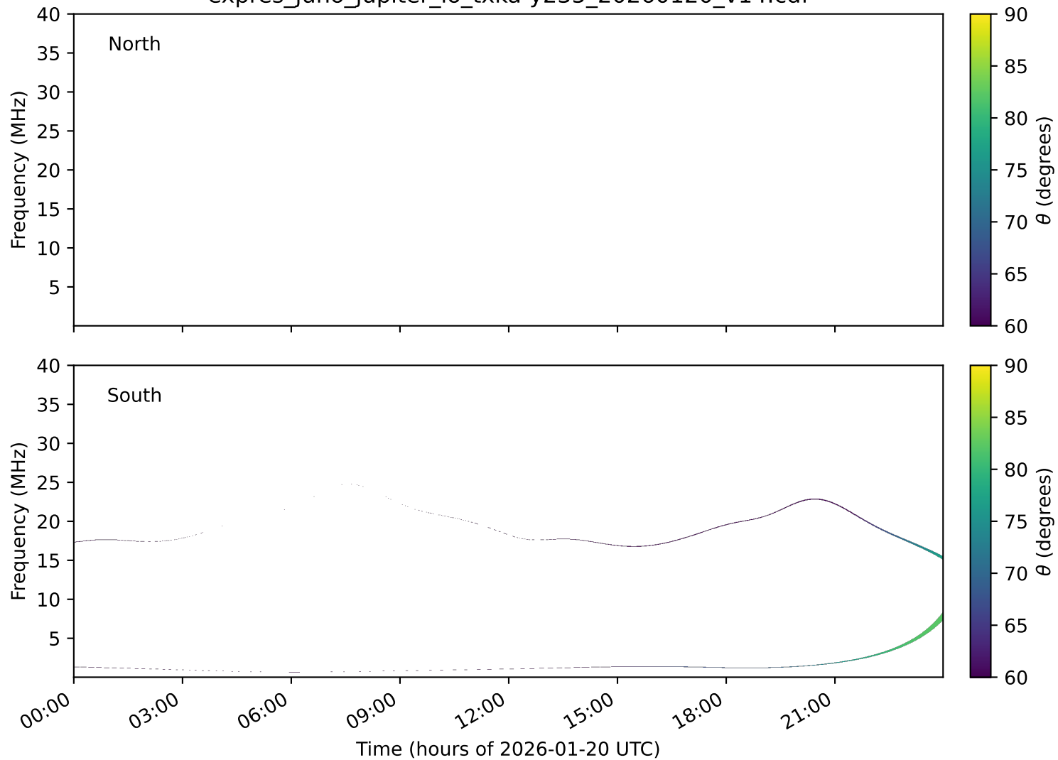
expres_juno_jupiter_io_txka-y235_20260120_v14.cdf
