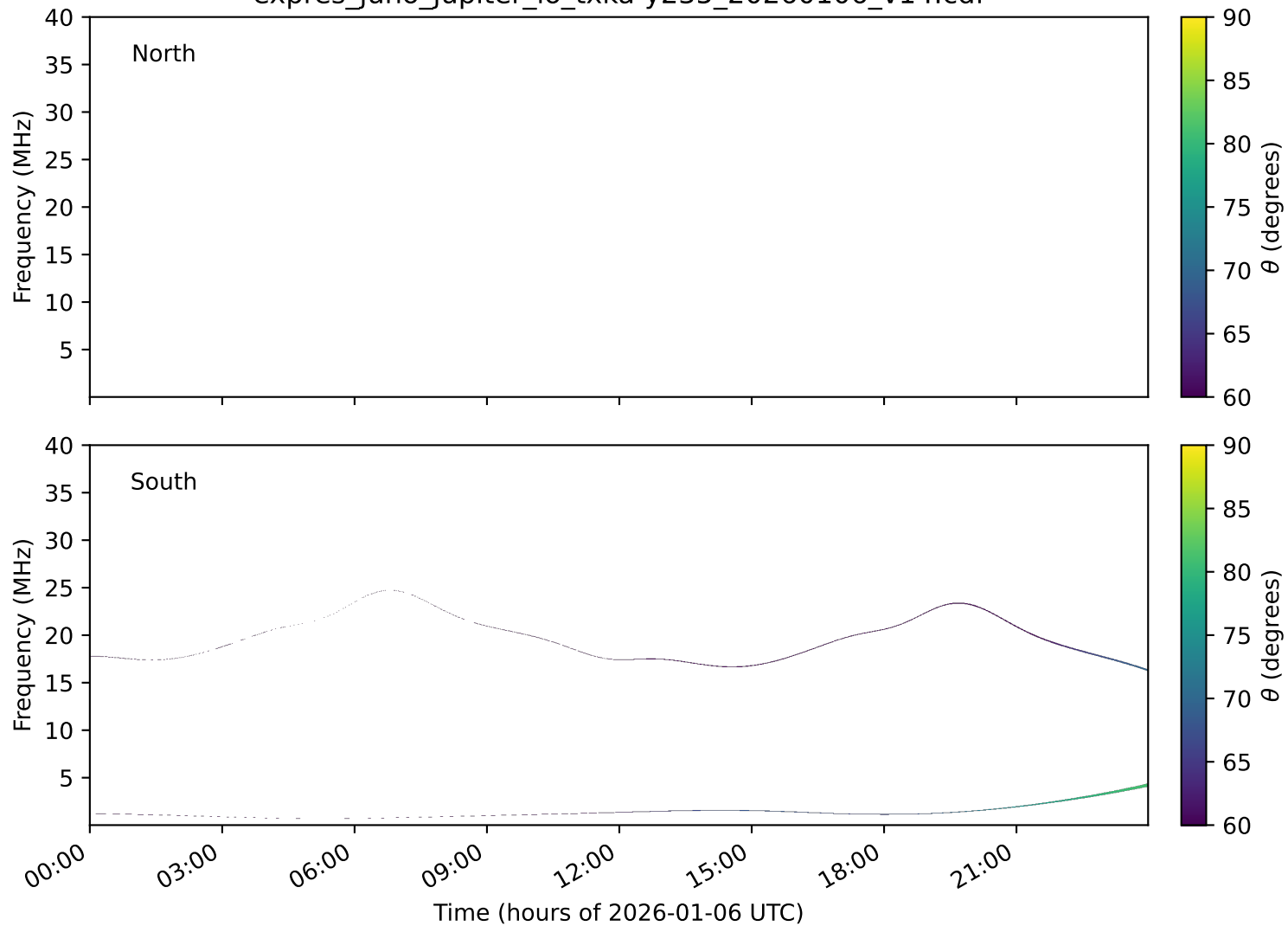
expres_juno_jupiter_io_txka-y235_20260106_v14.cdf
