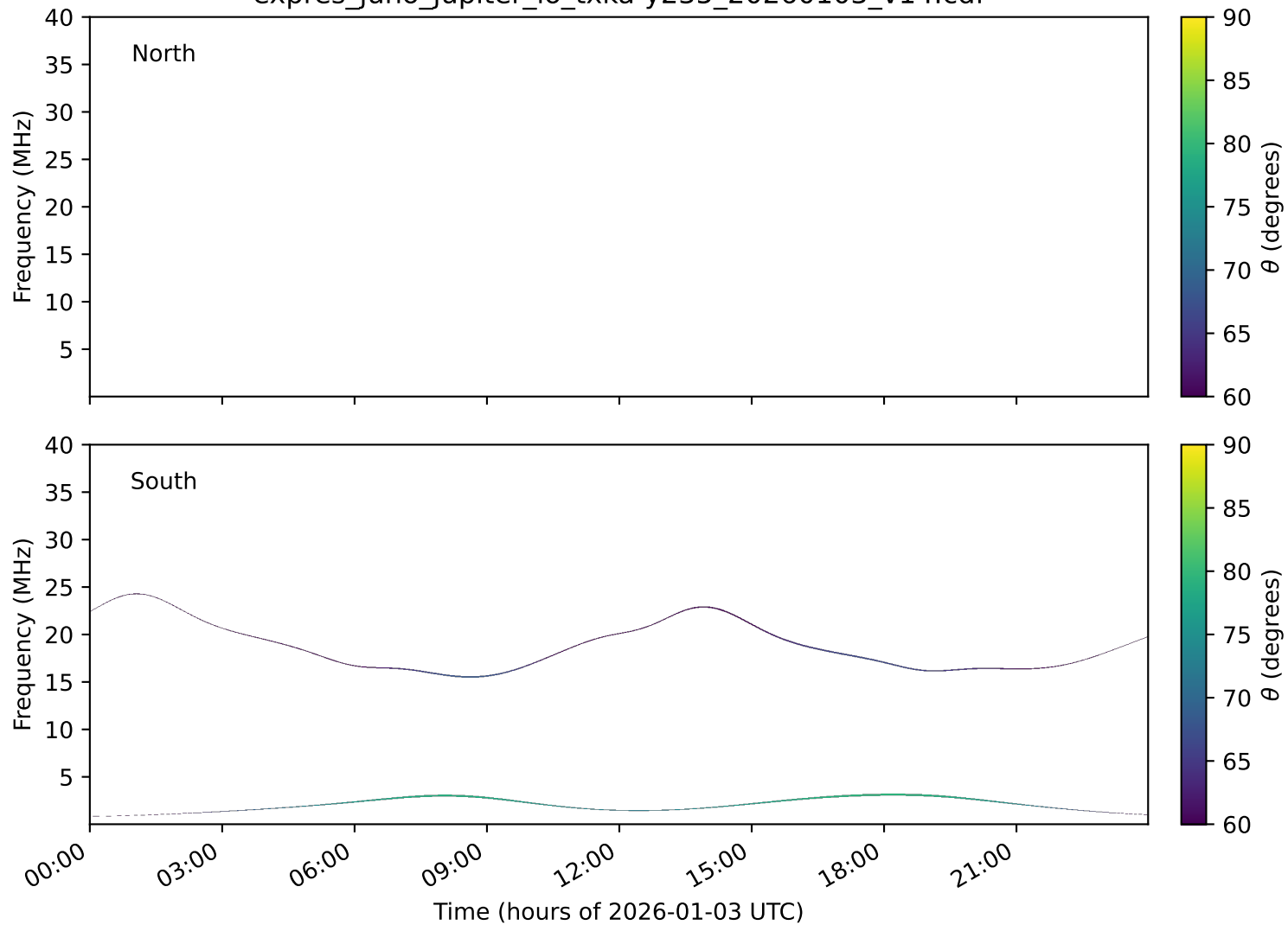
expres_juno_jupiter_io_txka-y235_20260103_v14.cdf
