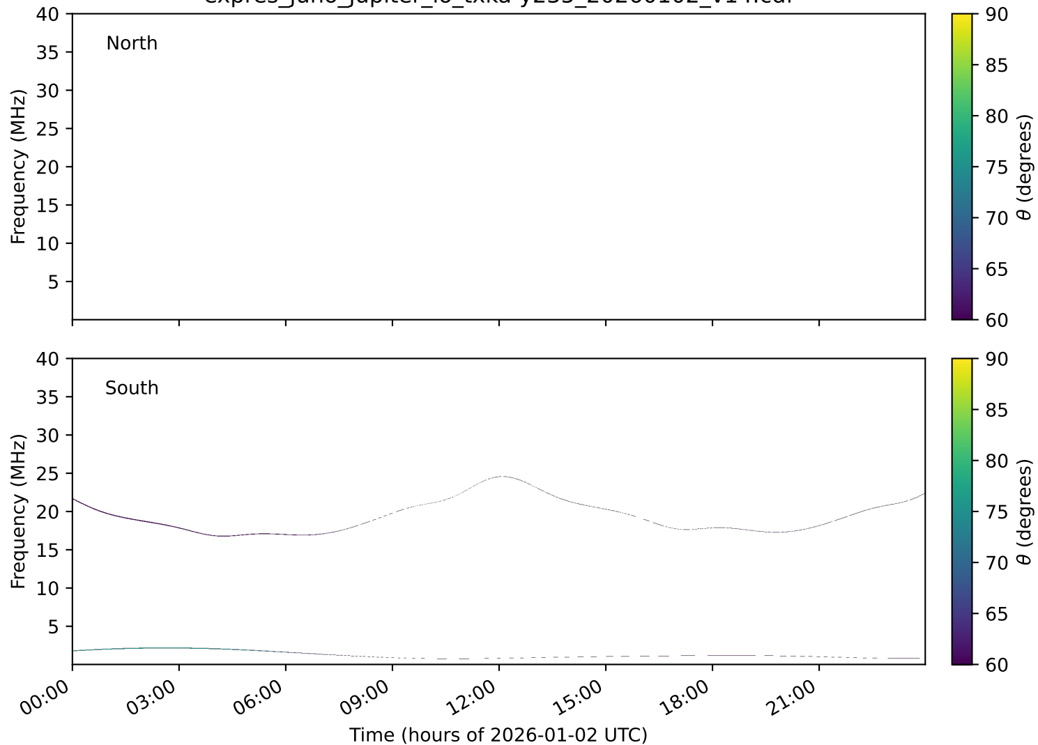
expres_juno_jupiter_io_txka-y235_20260102_v14.cdf
