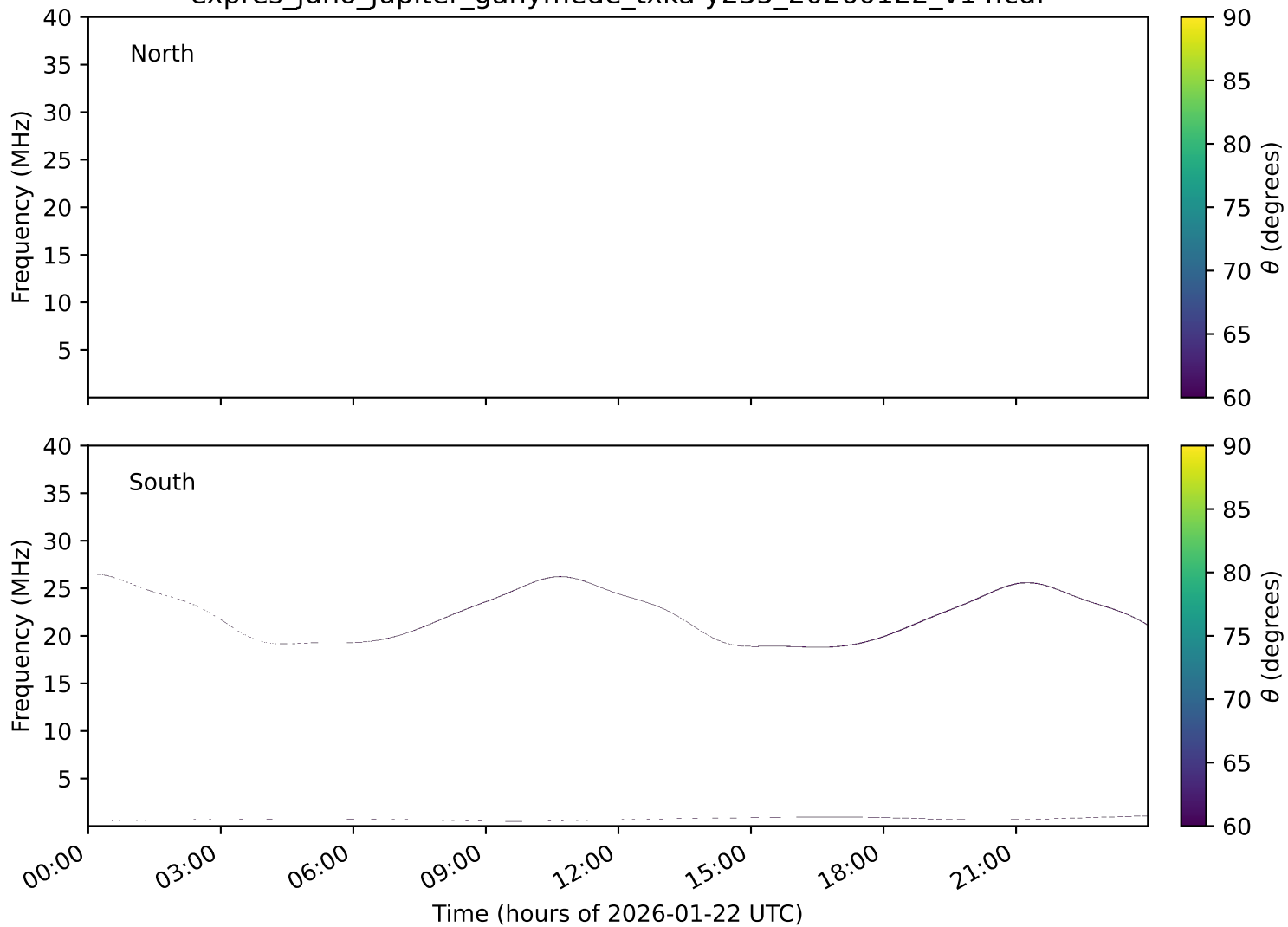
expres_juno_jupiter_ganymede_txka-y235_20260122_v14.cdf
