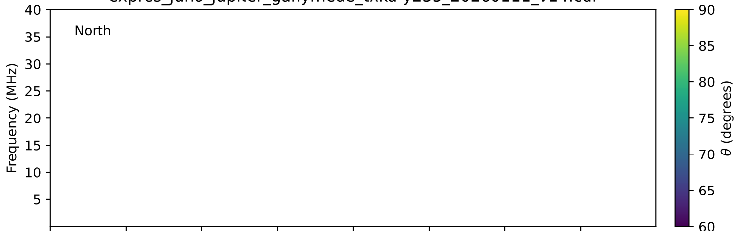
expres_juno_jupiter_ganymede_txka-y235_20260111_v14.cdf
