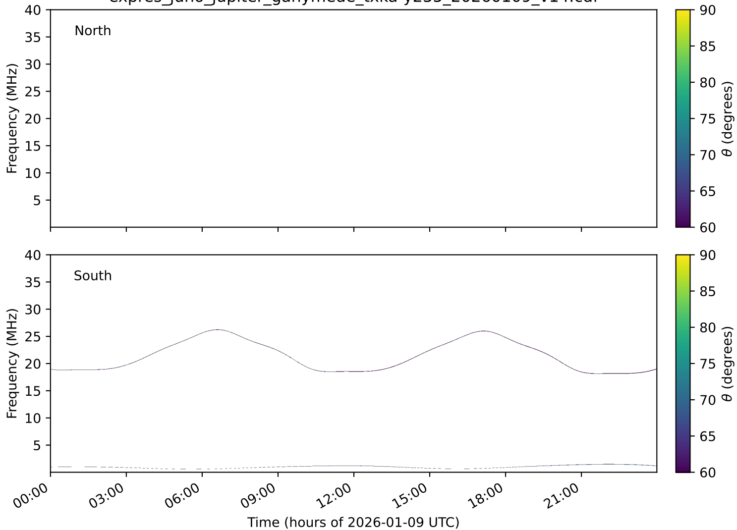
expres_juno_jupiter_ganymede_txka-y235_20260109_v14.cdf
