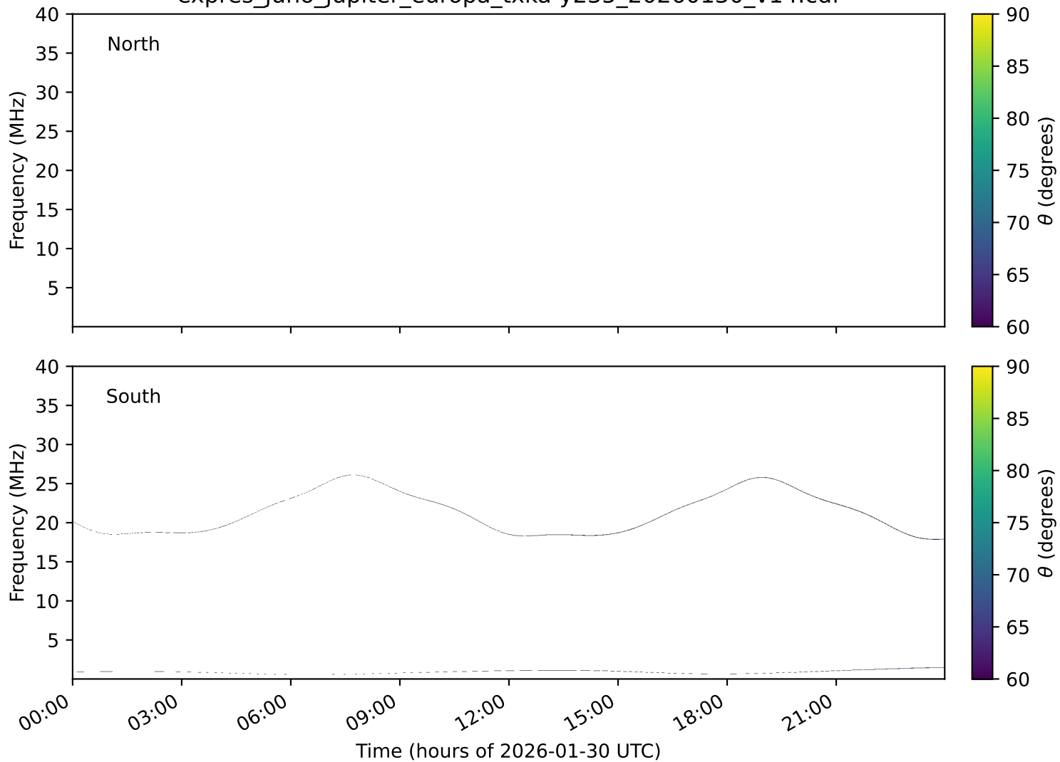
expres_juno_jupiter_europa_txka-y235_20260130_v14.cdf
