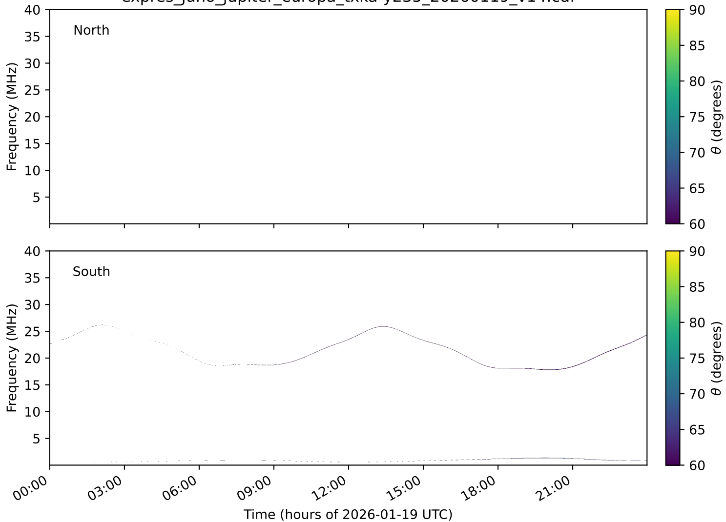
expres_juno_jupiter_europa_txka-y235_20260119_v14.cdf
