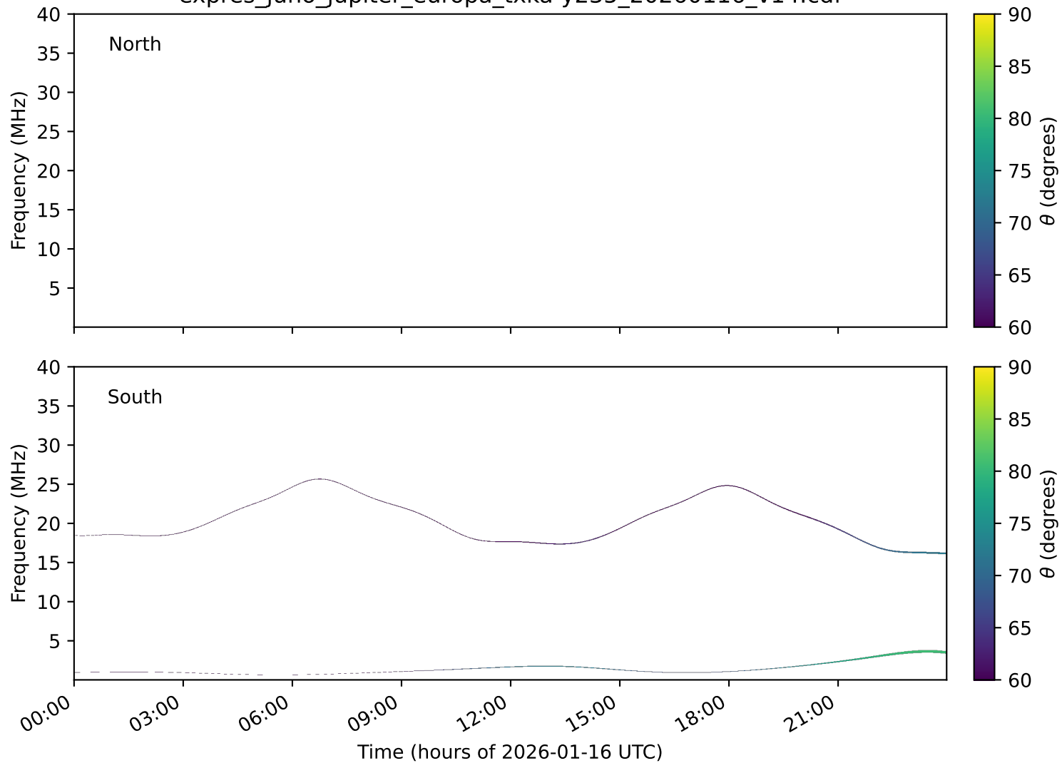
expres_juno_jupiter_europa_txka-y235_20260116_v14.cdf
