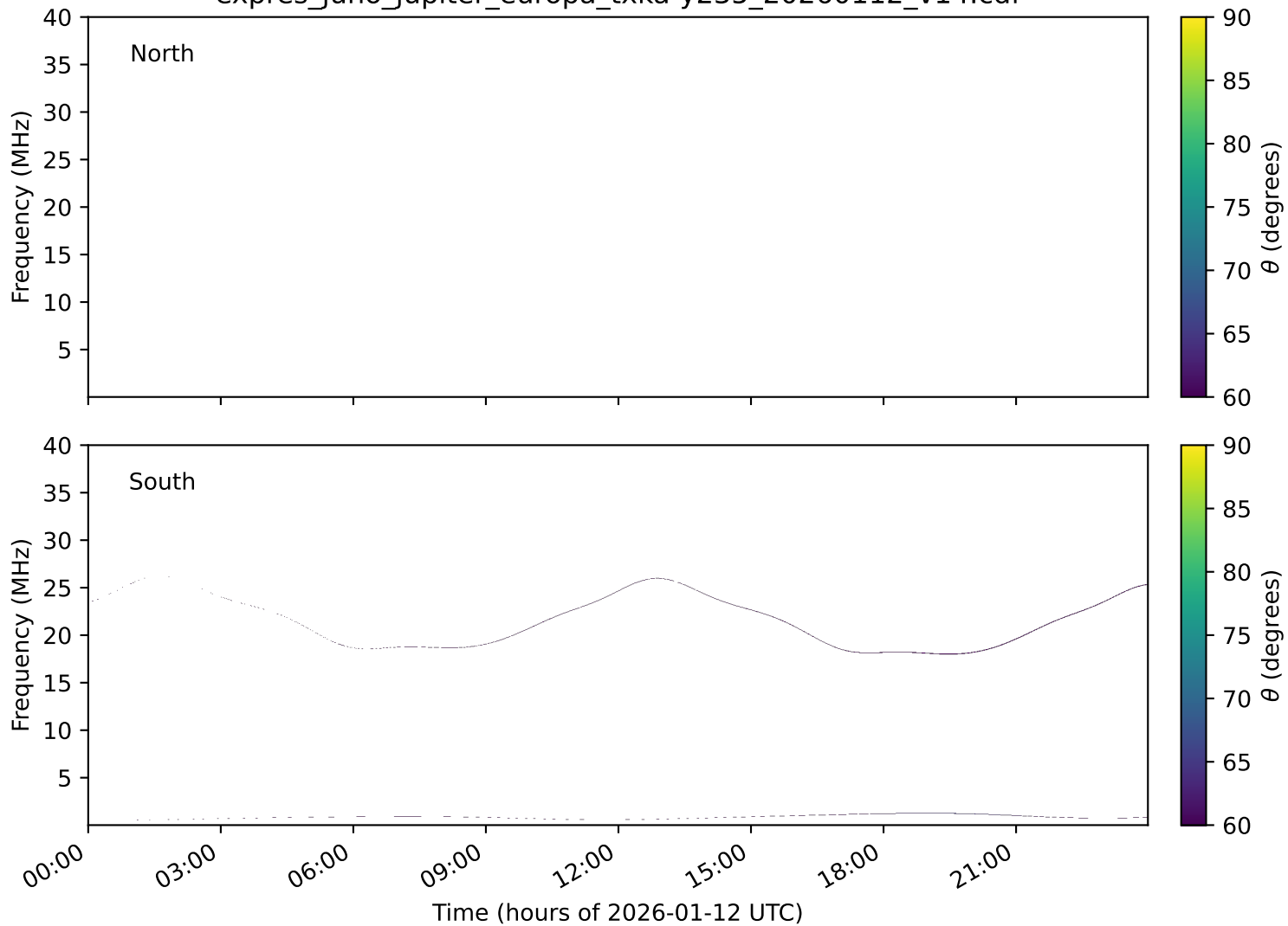
expres_juno_jupiter_europa_txka-y235_20260112_v14.cdf
