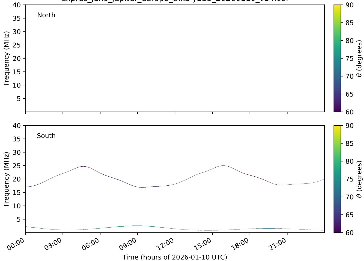
expres_juno_jupiter_europa_txka-y235_20260110_v14.cdf
