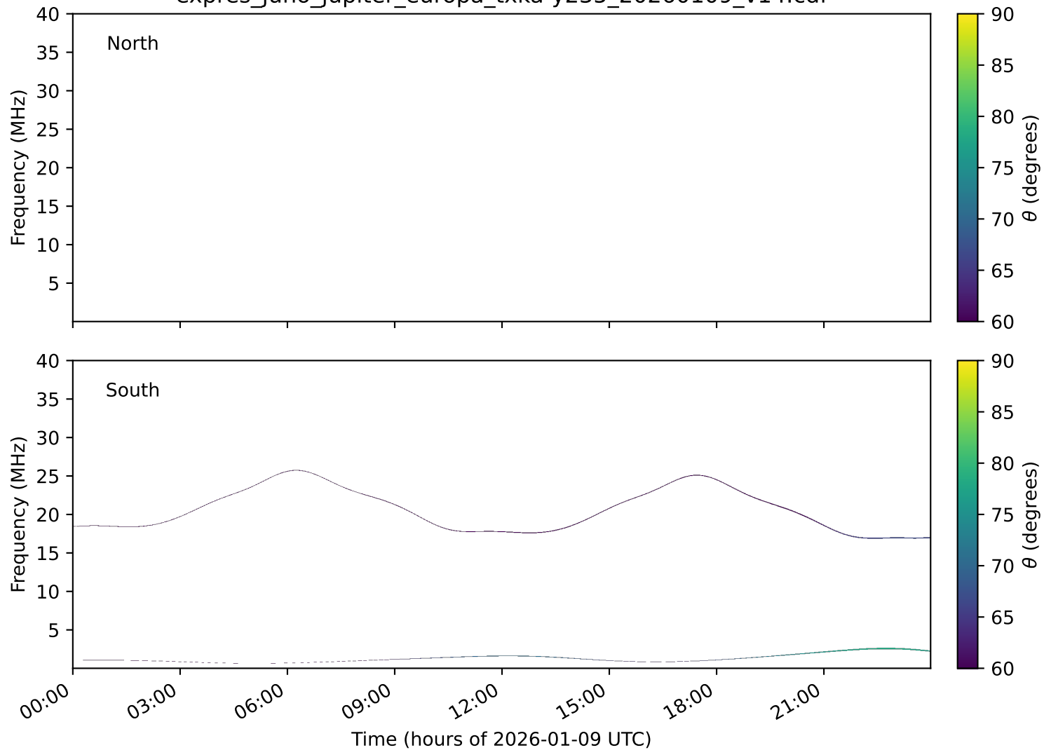
expres_juno_jupiter_europa_txka-y235_20260109_v14.cdf
