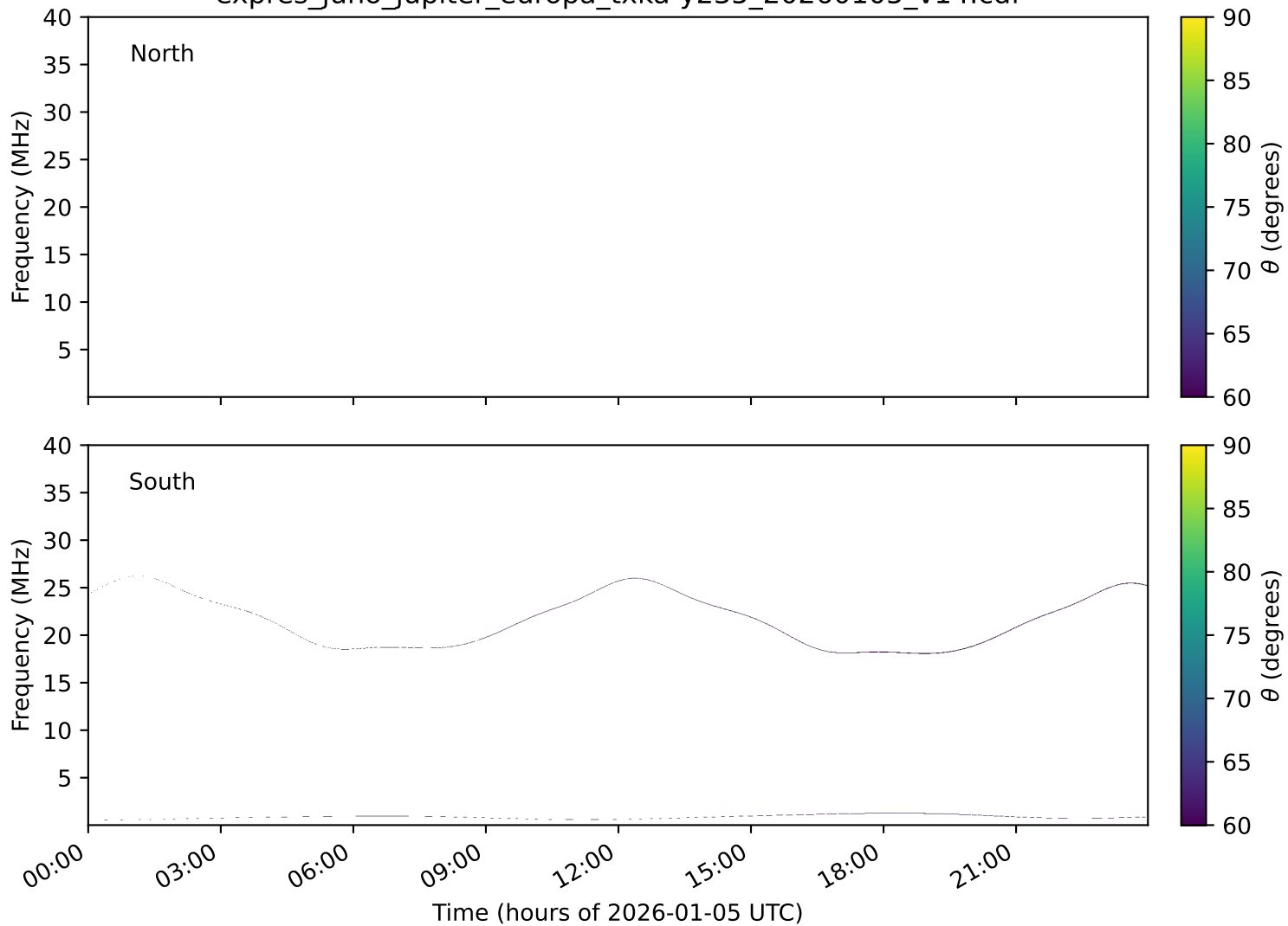
expres_juno_jupiter_europa_txka-y235_20260105_v14.cdf
