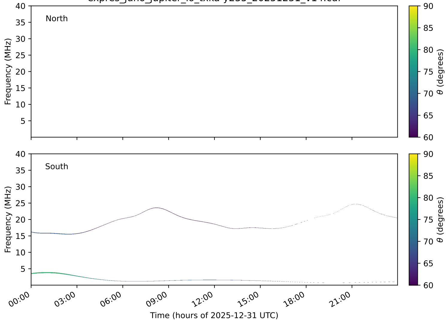
expres_juno_jupiter_io_txka-y235_20251231_v14.cdf
