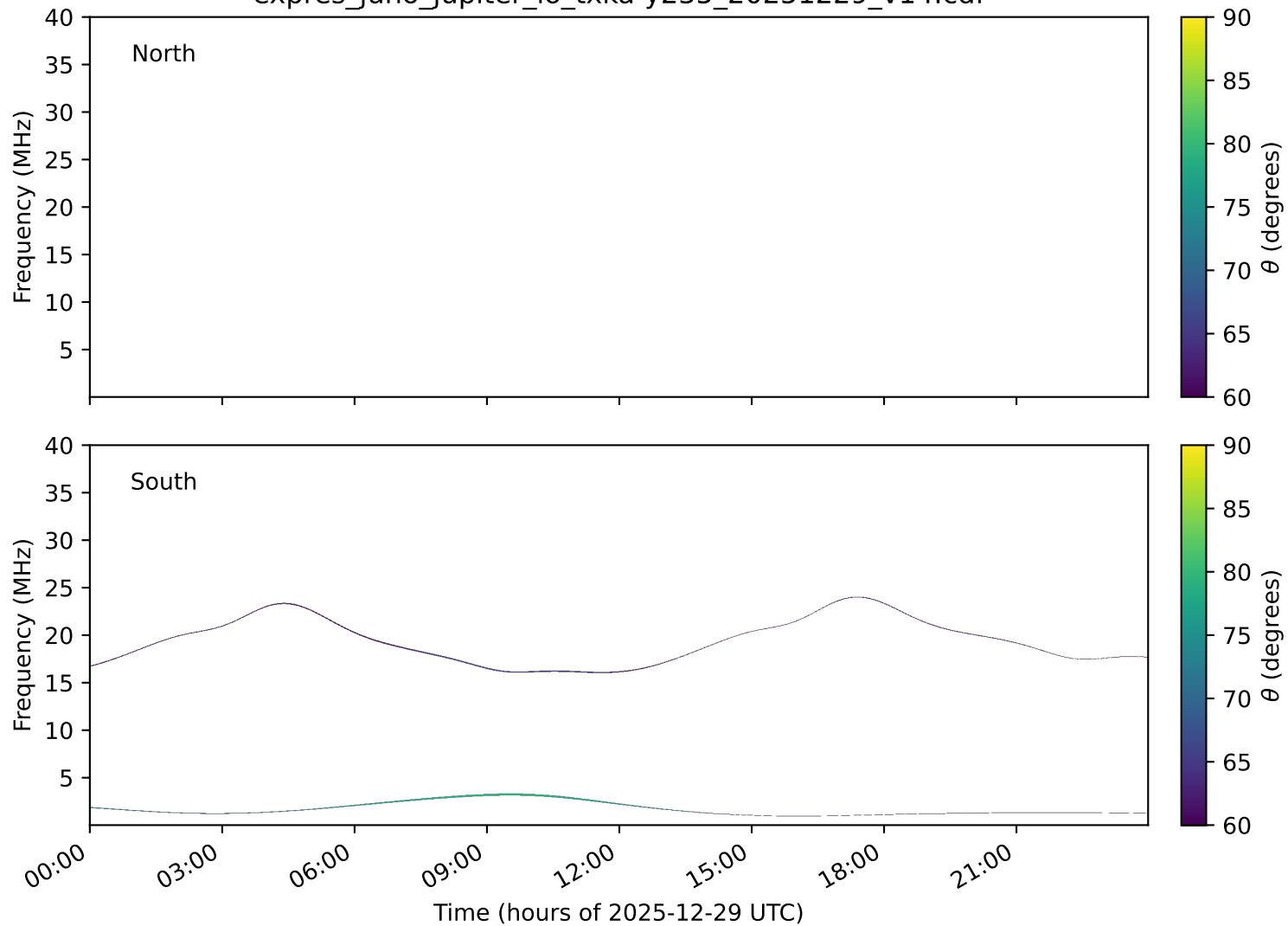
expres_juno_jupiter_io_txka-y235_20251229_v14.cdf
