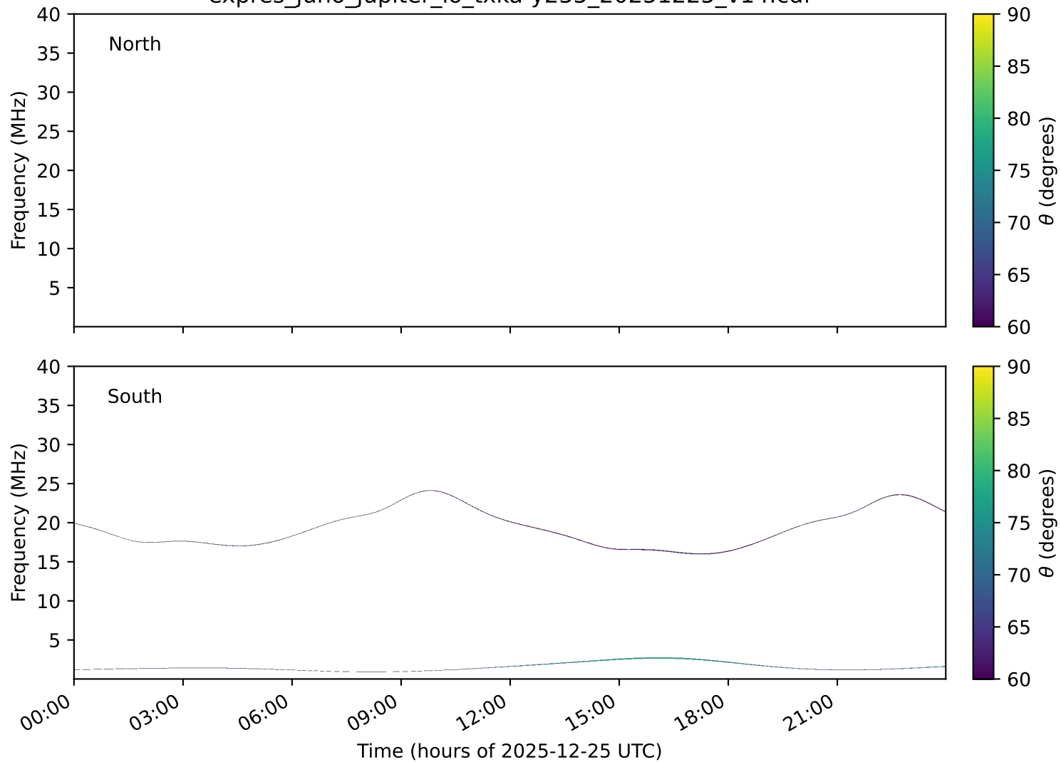
expres_juno_jupiter_io_txka-y235_20251225_v14.cdf
