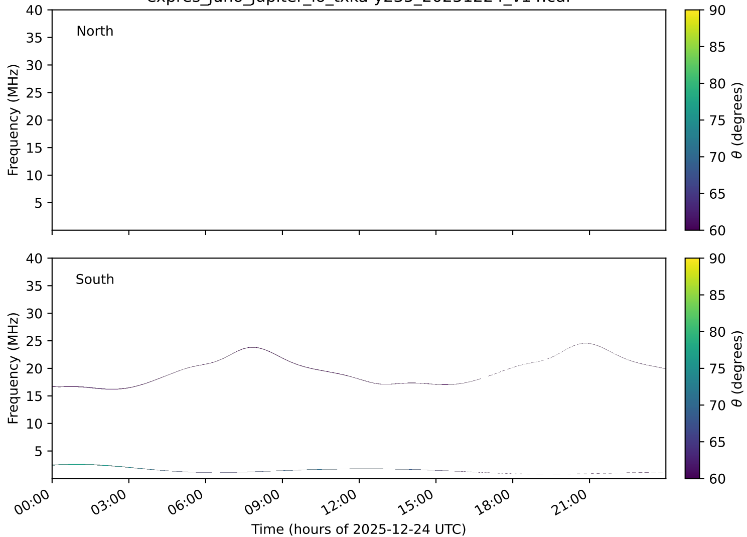
expres_juno_jupiter_io_txka-y235_20251224_v14.cdf
