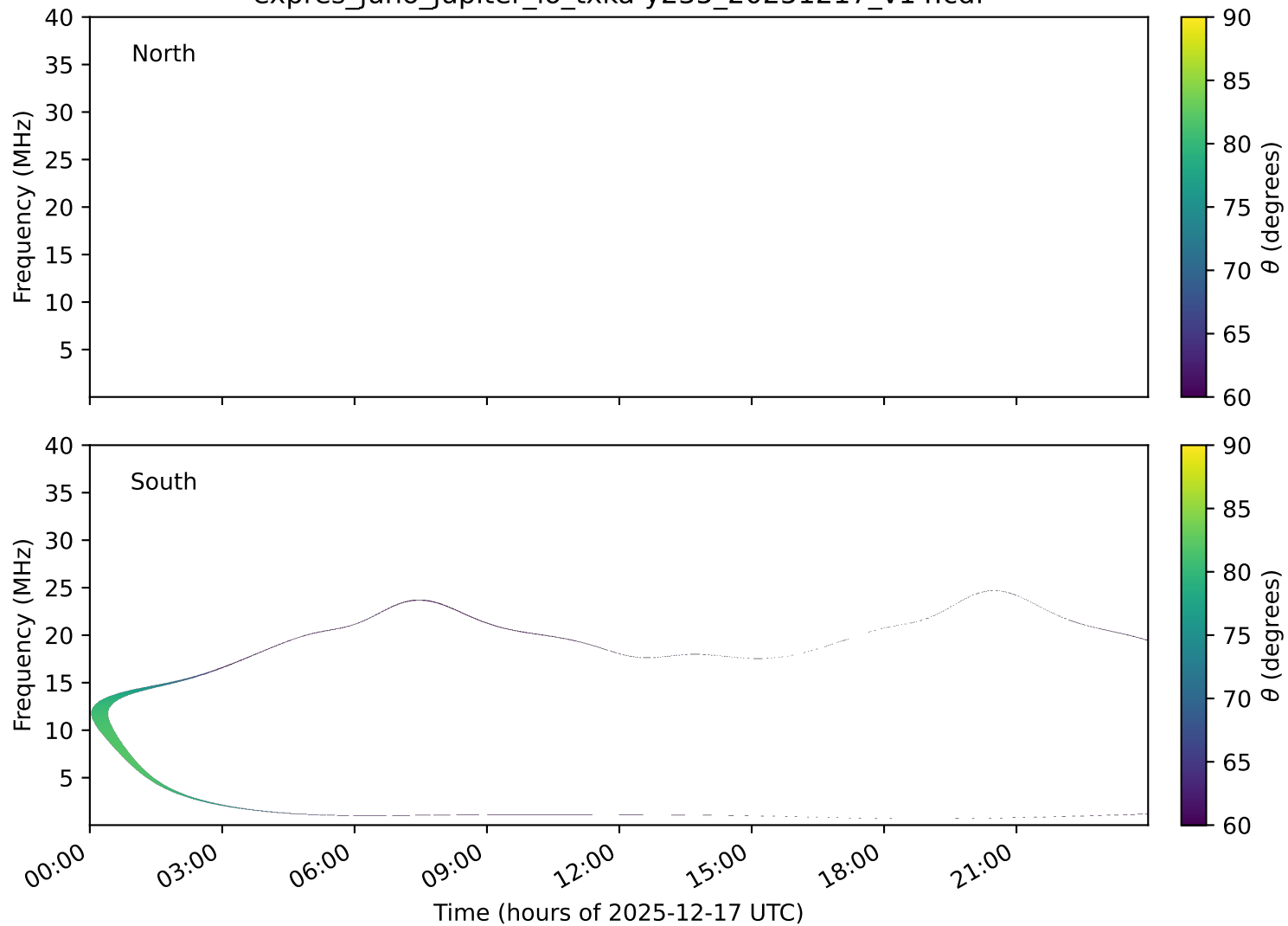
expres_juno_jupiter_io_txka-y235_20251217_v14.cdf
