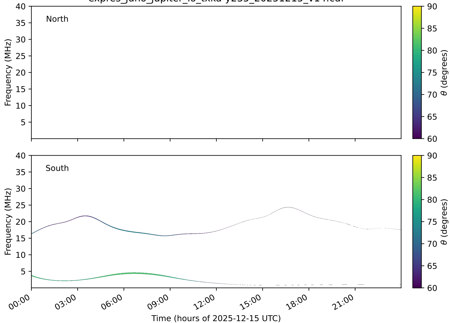
expres_juno_jupiter_io_txka-y235_20251215_v14.cdf
