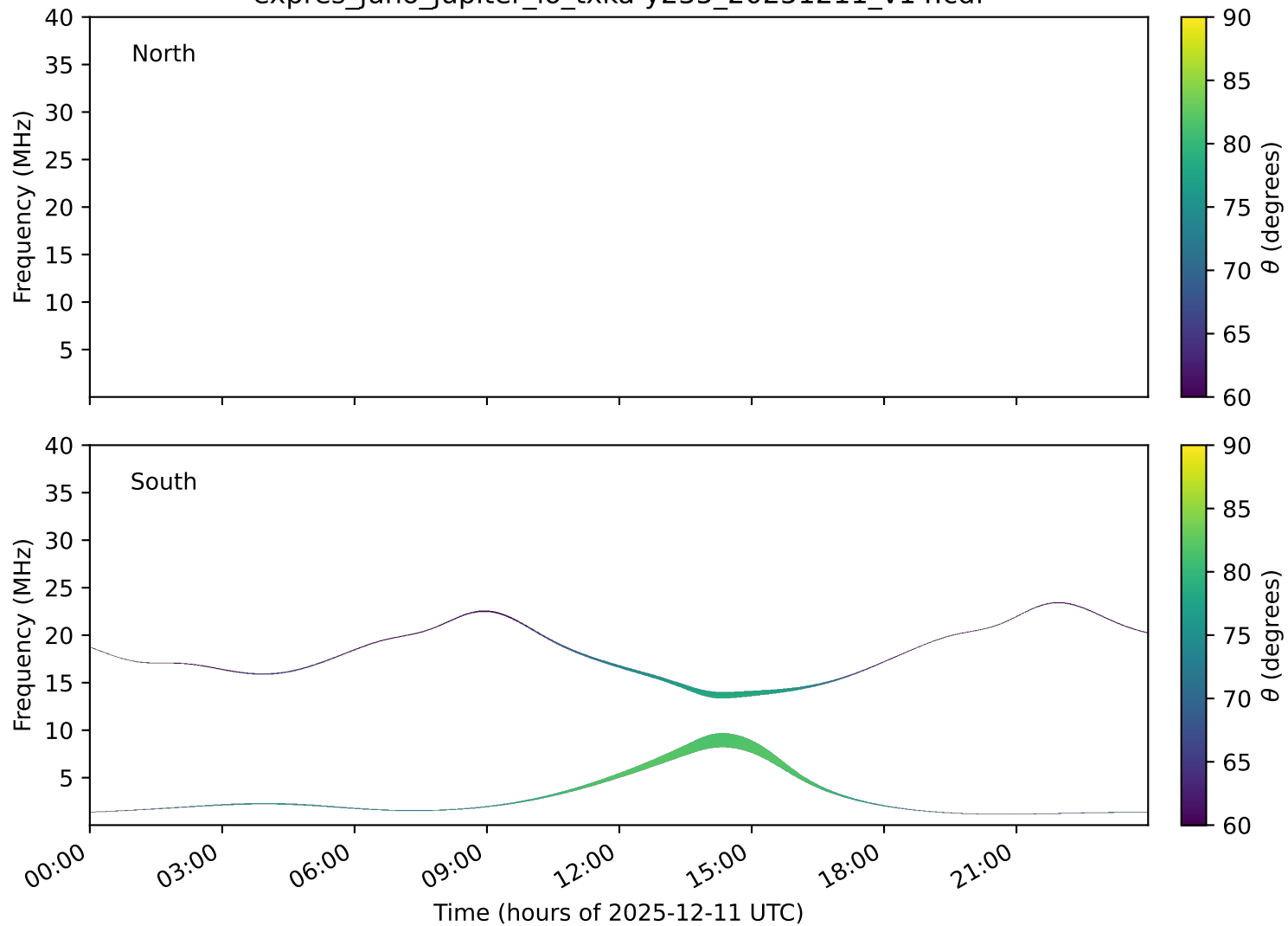
expres_juno_jupiter_io_txka-y235_20251211_v14.cdf
