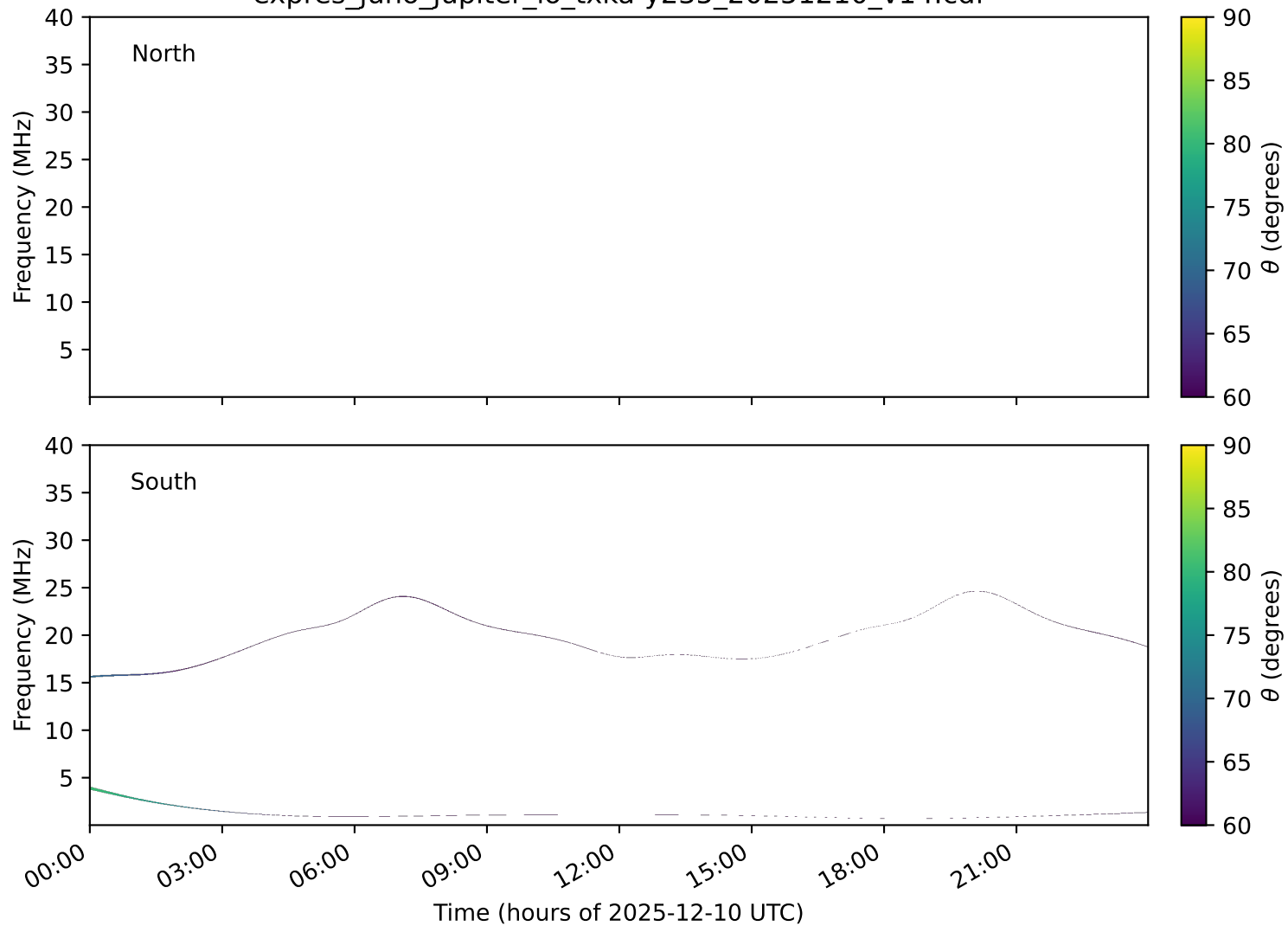
expres_juno_jupiter_io_txka-y235_20251210_v14.cdf
