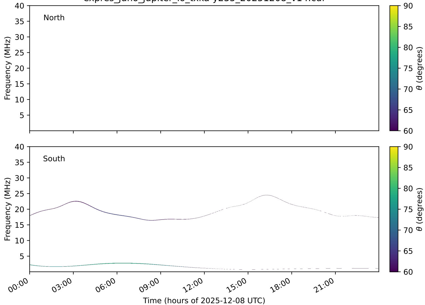
expres_juno_jupiter_io_txka-y235_20251208_v14.cdf
