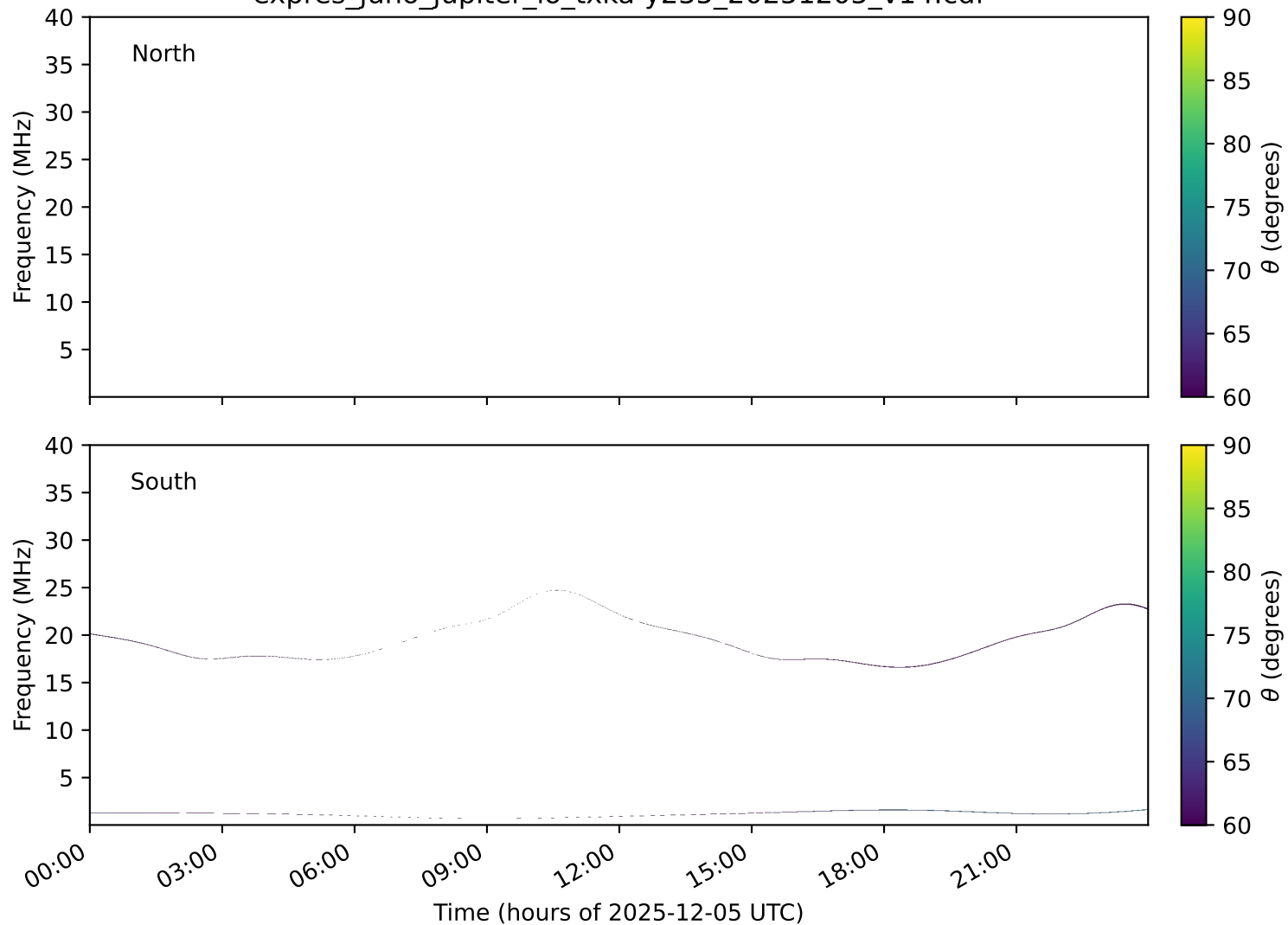
expres_juno_jupiter_io_txka-y235_20251205_v14.cdf
