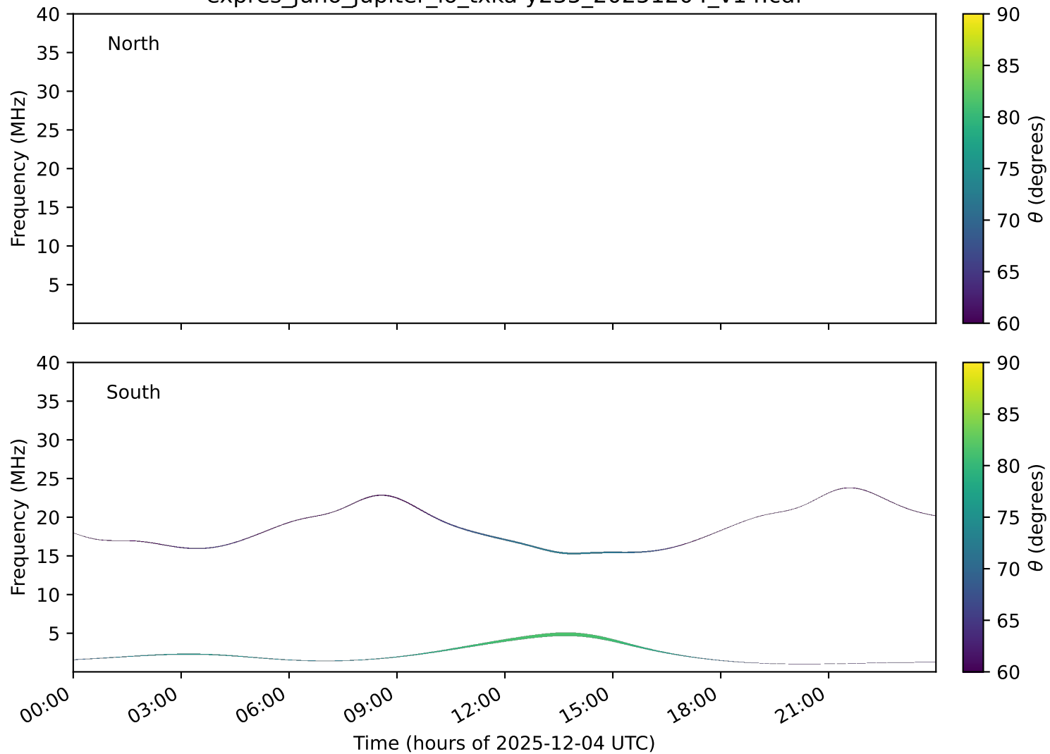
expres_juno_jupiter_io_txka-y235_20251204_v14.cdf
